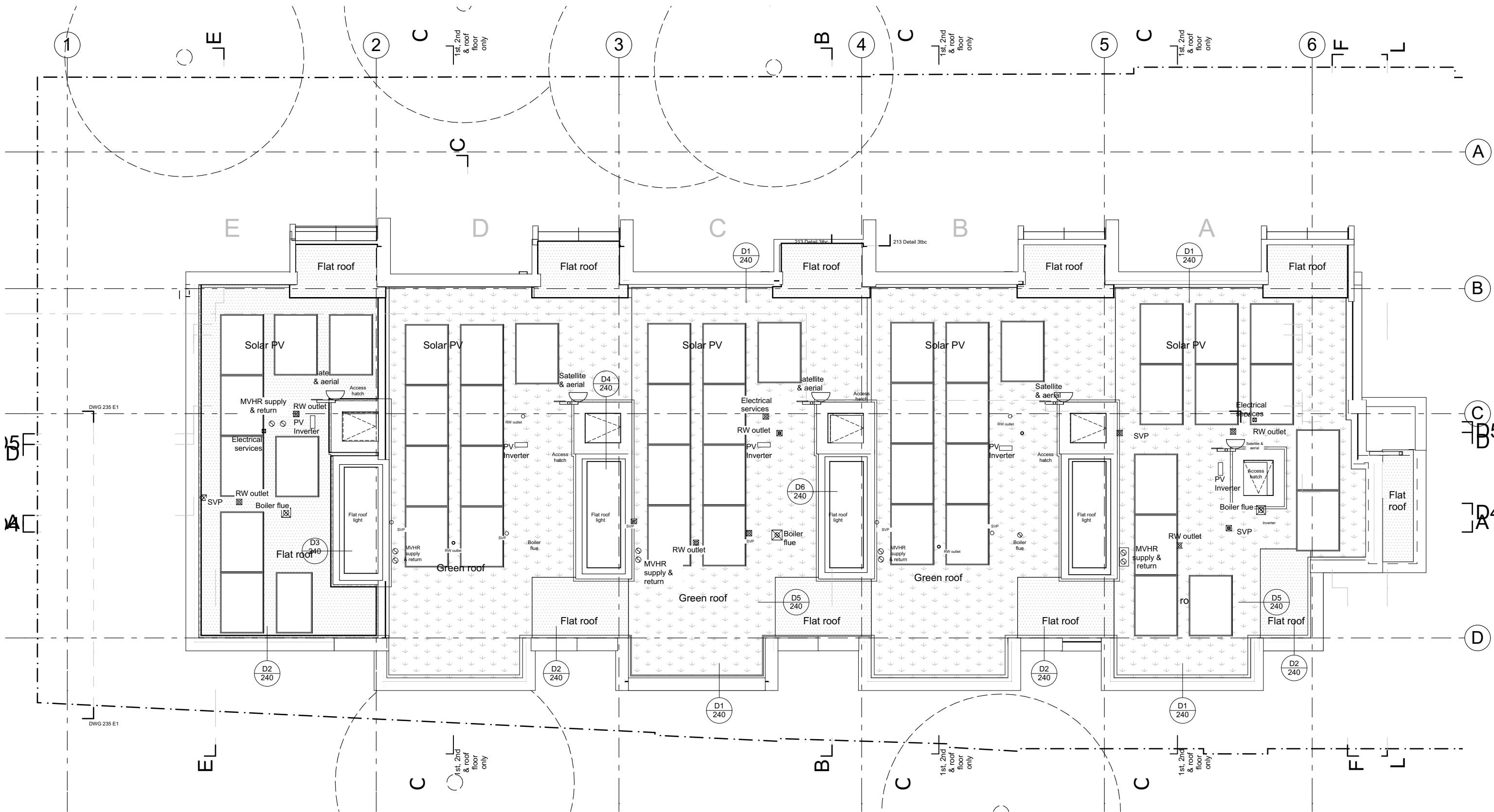
Roof Scale @A3 - 1:100
