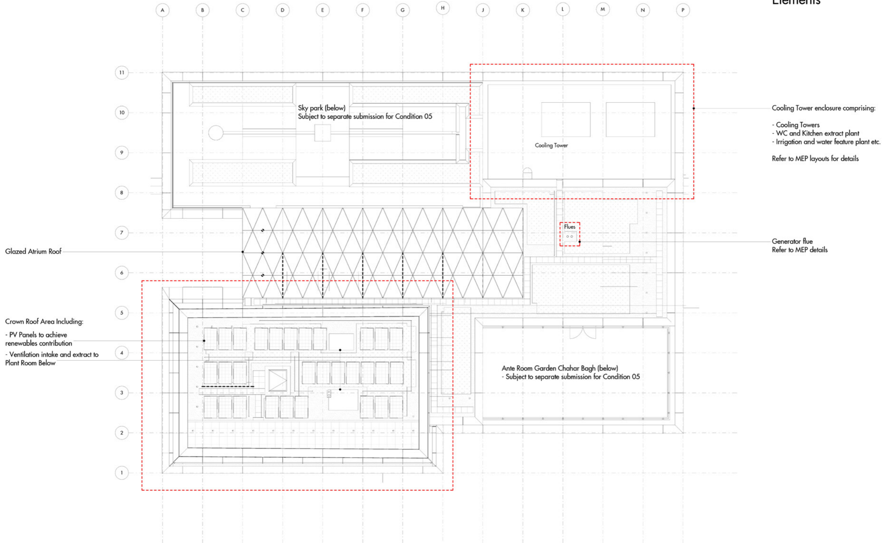
1.1 - ROOF OVERVIEW PLAN
