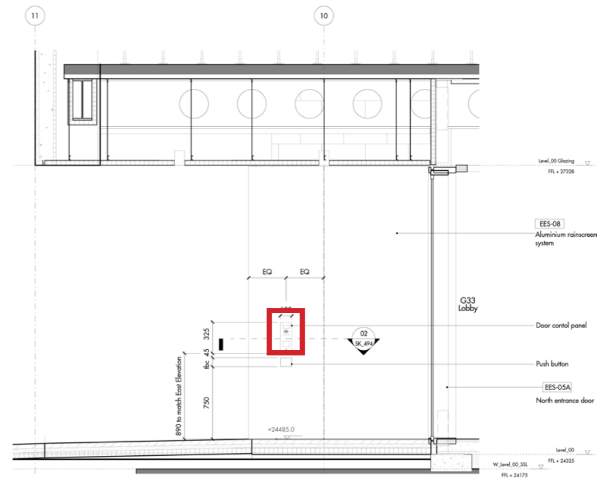
ELEVATION - INTERCOM UNIT AT NORTH ENTRANCE
