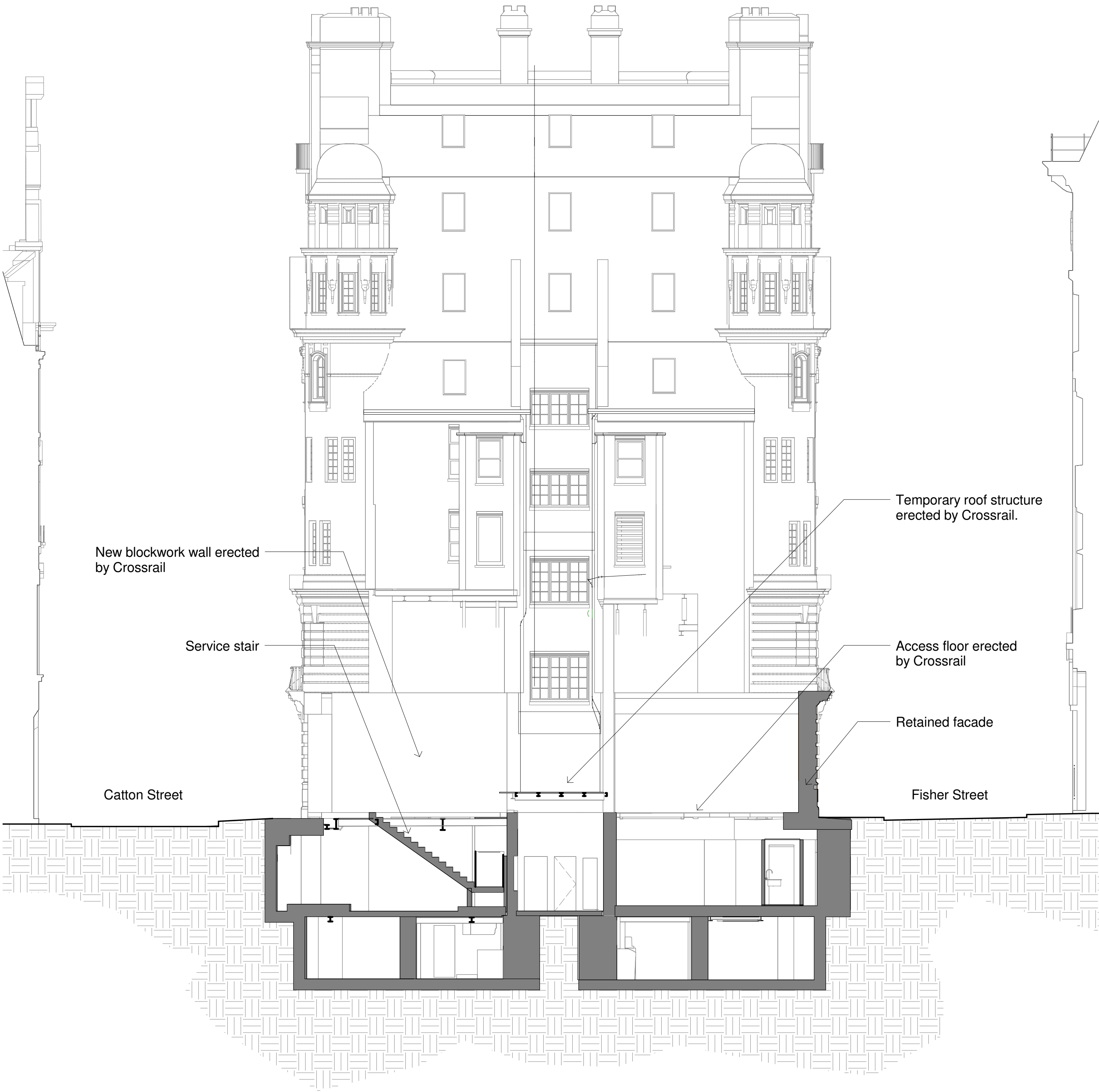
1 Existing Section BB Scale 1 : 100
