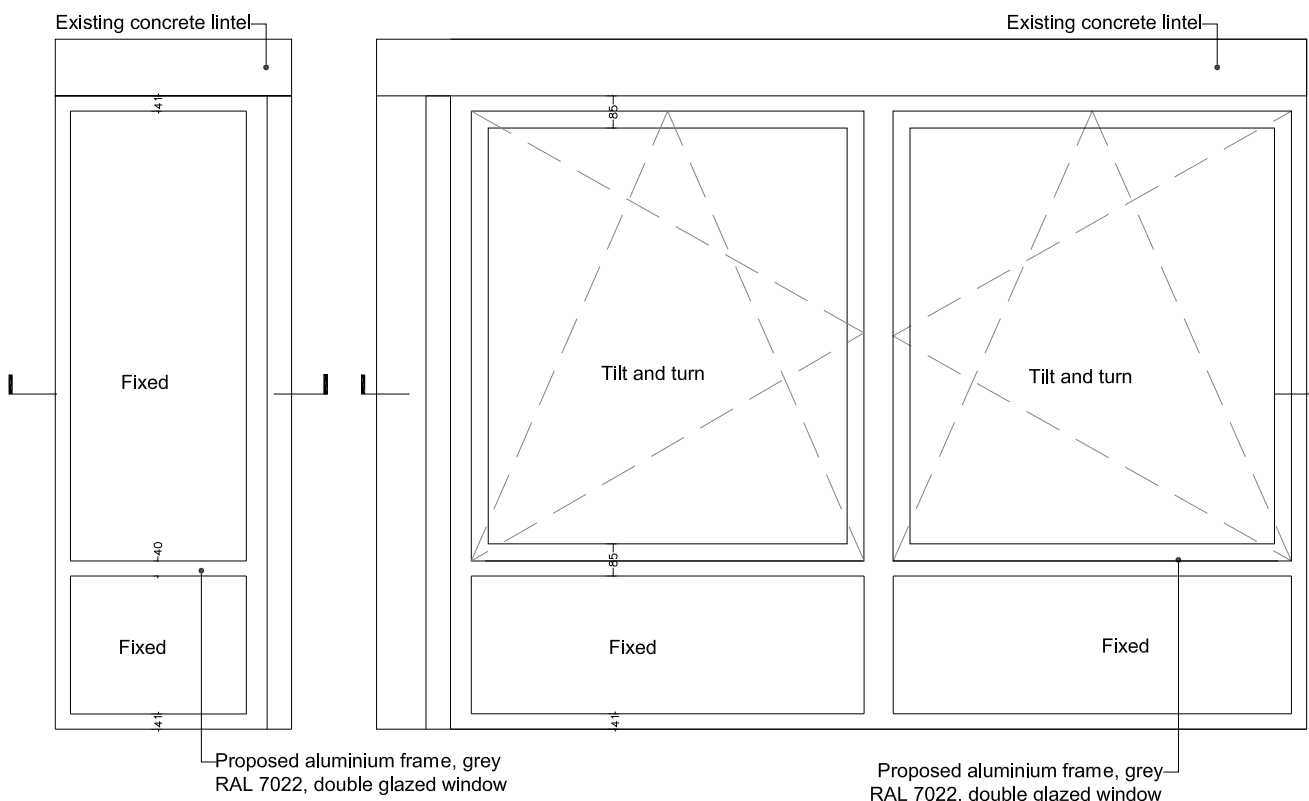
Proposed elevation of typical corner window
