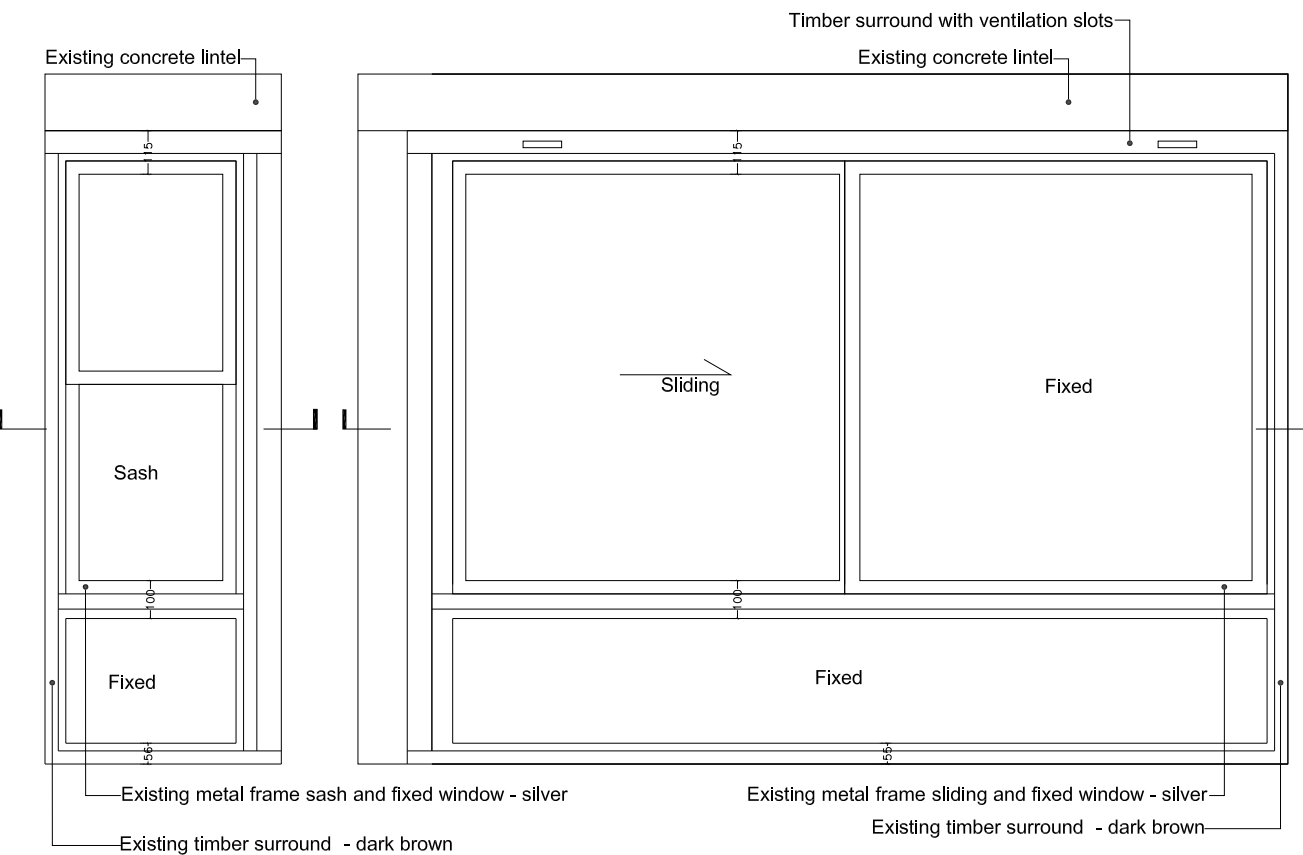
Existing elevation of typical corner window
