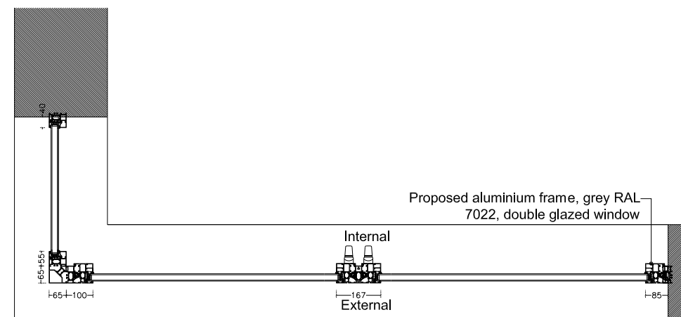
Proposed plan of typical window
