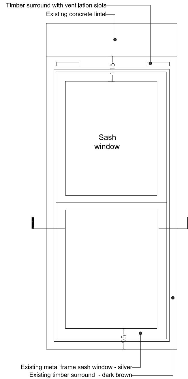
Existing elevation of typical window
