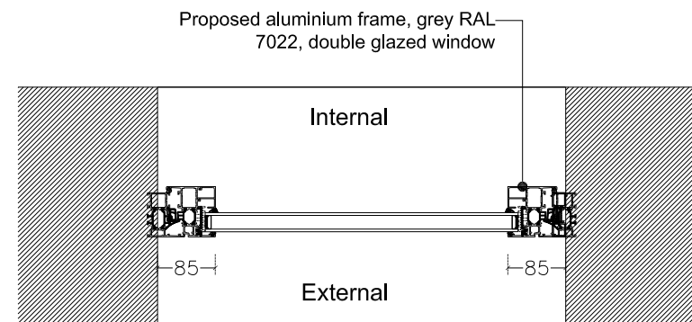
Proposed plan of typical window
