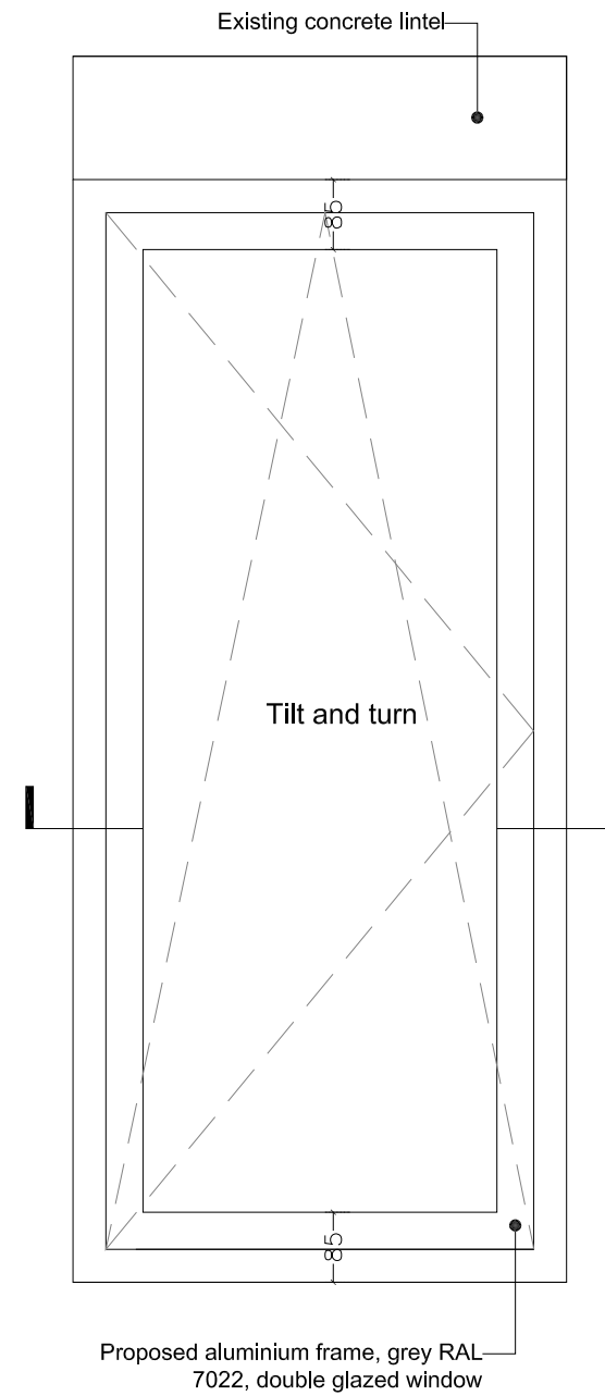
Proposed elevation of typical window
