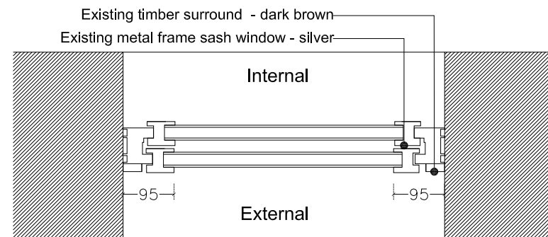
Existing plan of typical window
