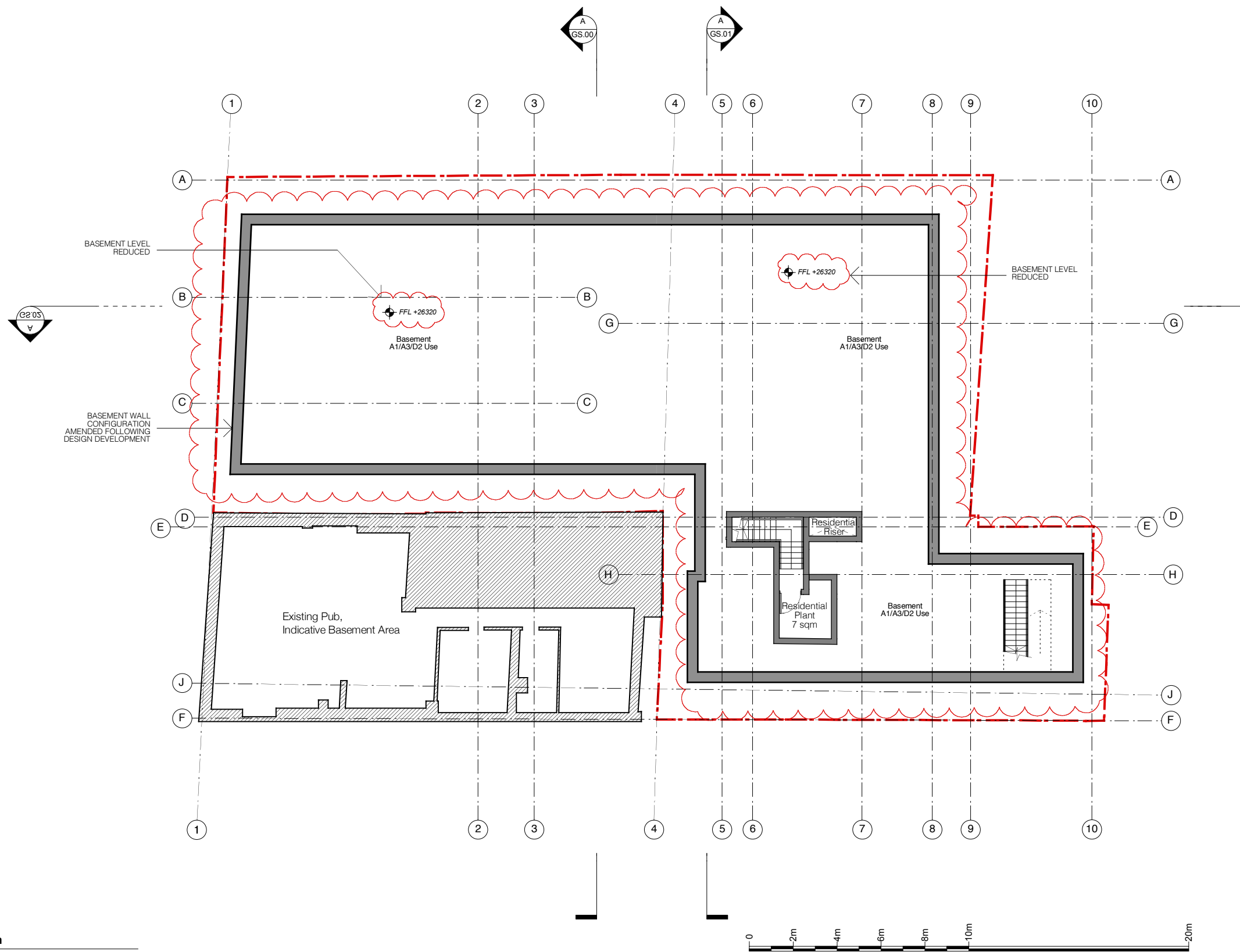
B Basement Floor Plan GA-01S 1:200@A3_1:100@A1
