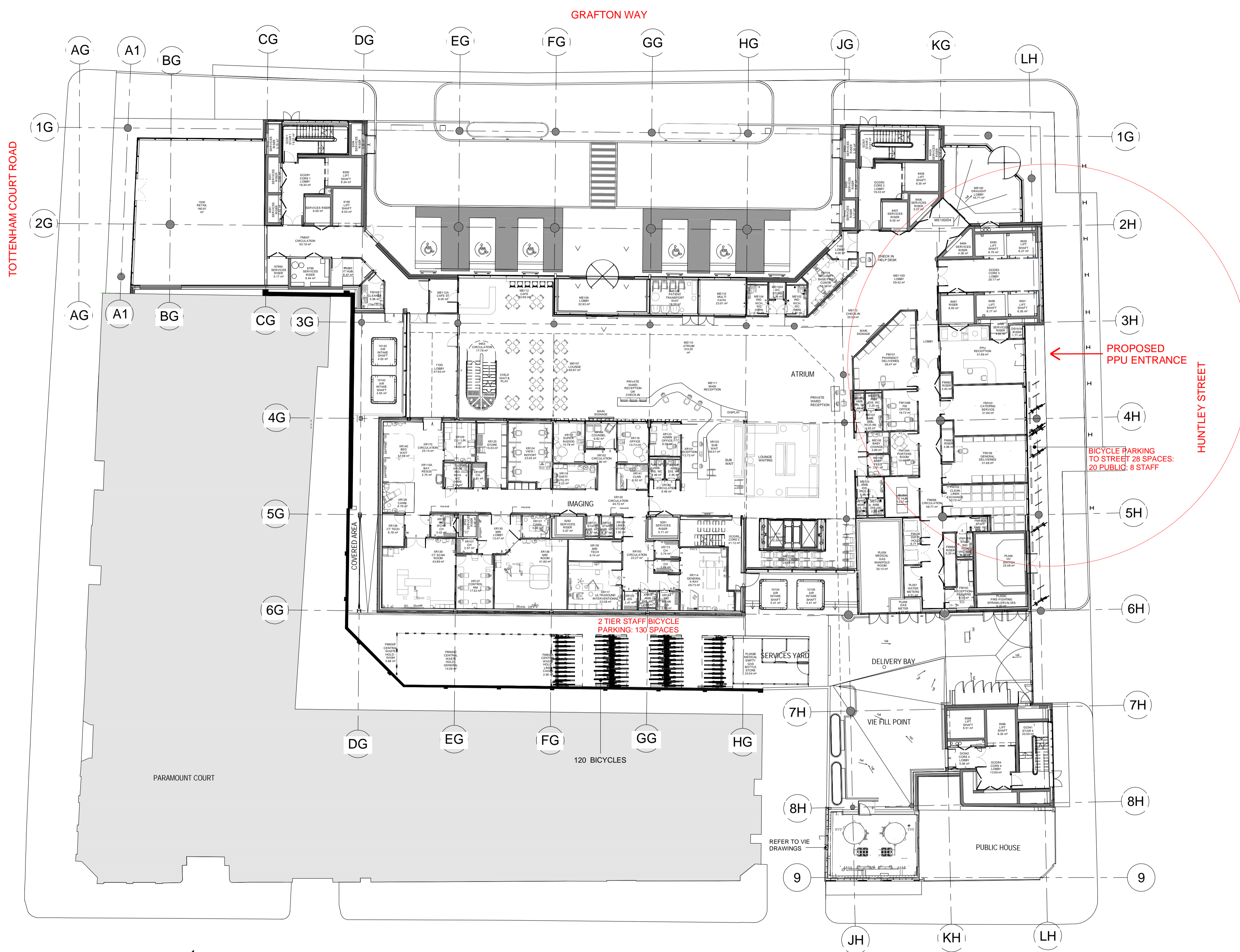
1 Ground Floor Level 111071 1:200
