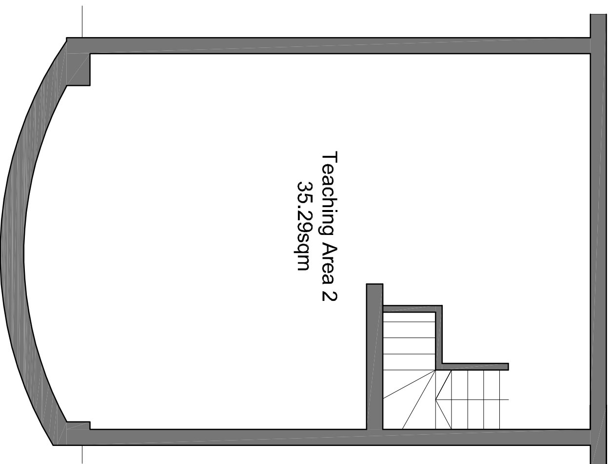
EXISTING & PROPOSED BASEMENT FLOOR PLAN
