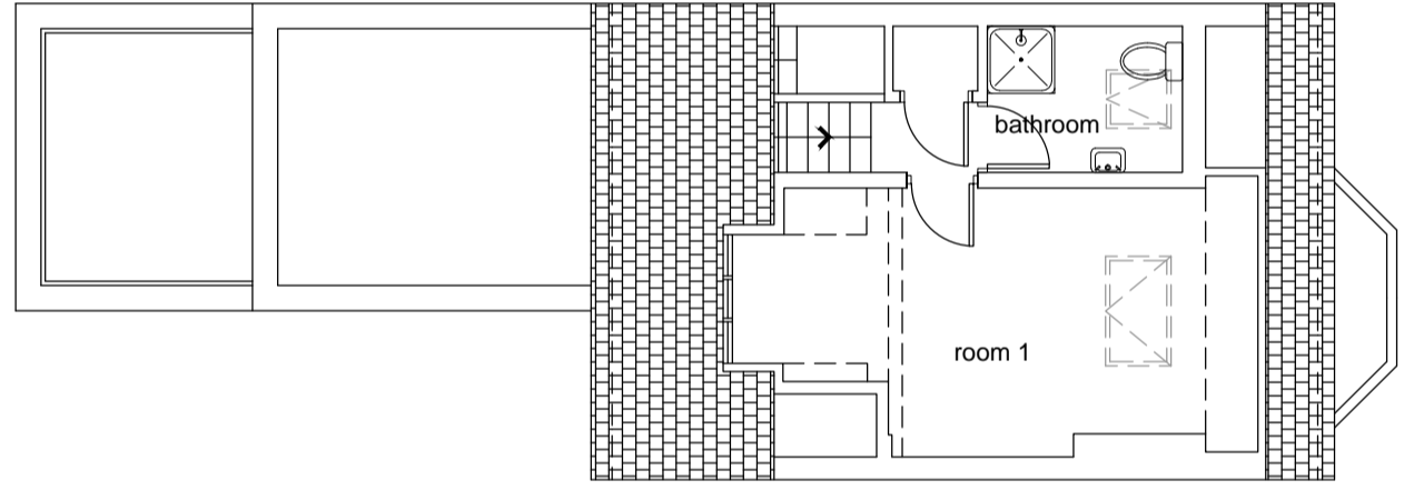
Existing Loft
