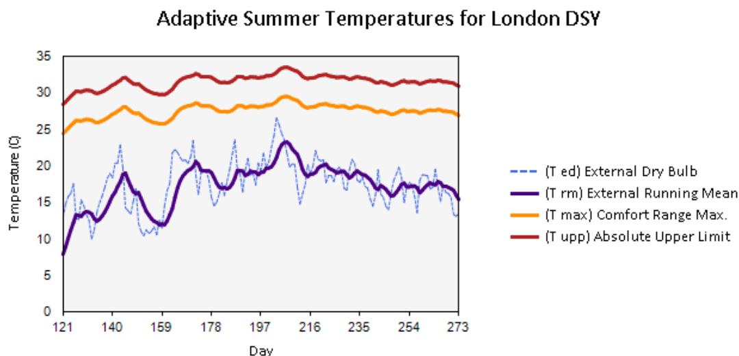
Figure 21 – CIBSE TM 52 Adaptive Summer Temperatures for London DSY
