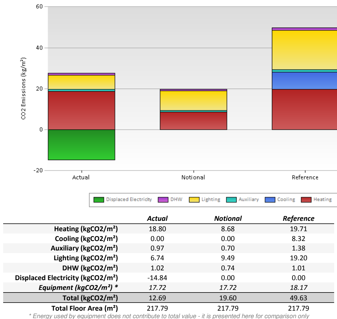
Figure 19 – Chart Comparing the Emissions for the Actual, Notional and Reference Buildings for the Entire Development at the 'Be Green' Stage of the Energy Hierarchy
