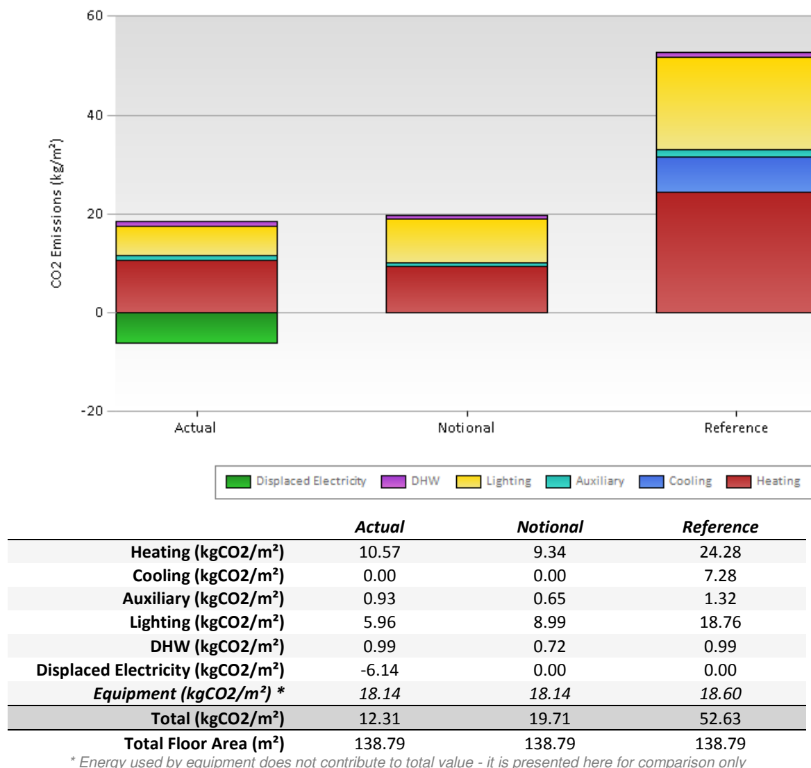
Figure 20 – Chart Comparing the Emissions for the Actual. Notional and Reference Buildings for the New Extension Only at the 'Be Green' Stage of the Energy Hierarchy
