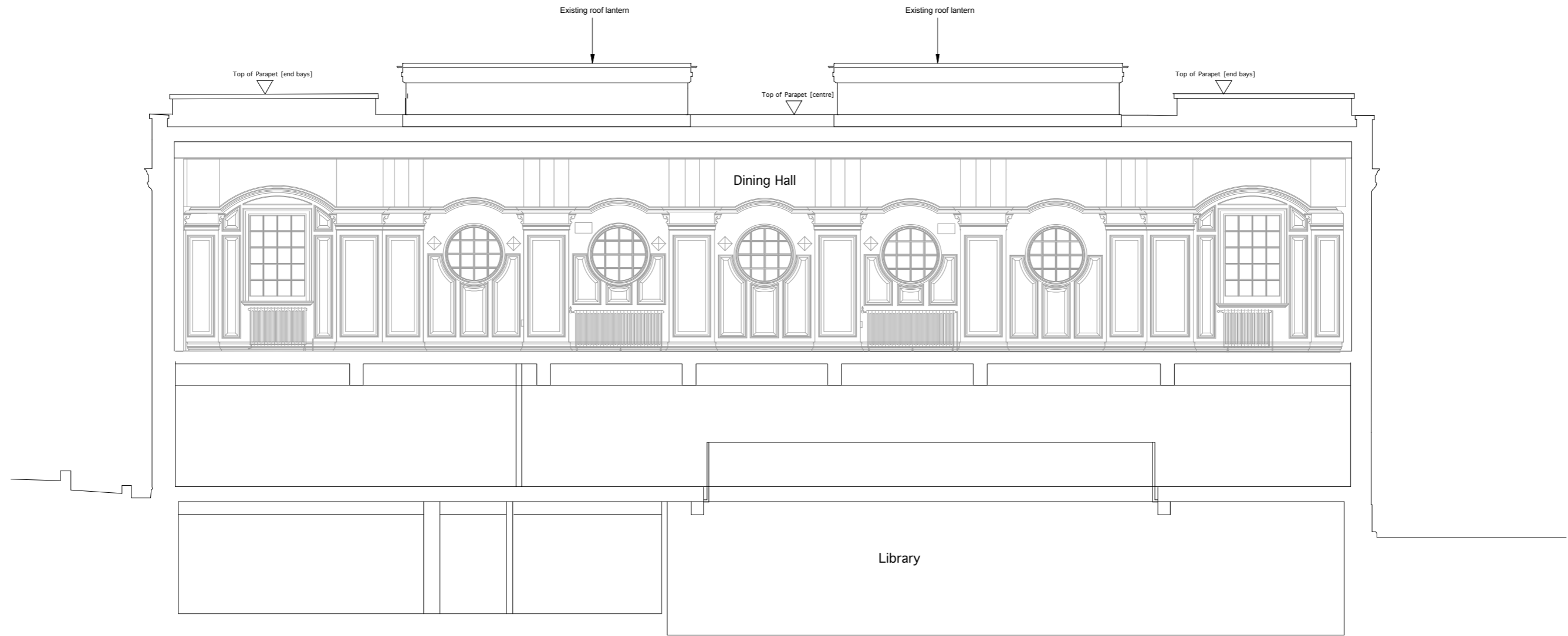
Section E-E
