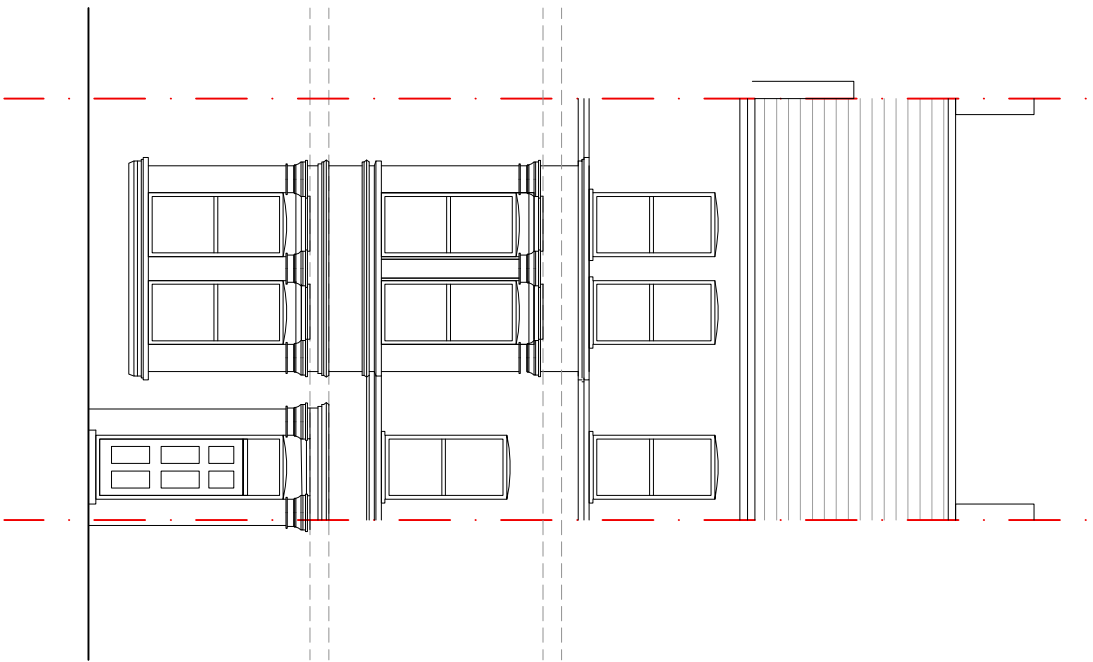
PROPOSED FRONT ELEVATION (NO CHANGES)
