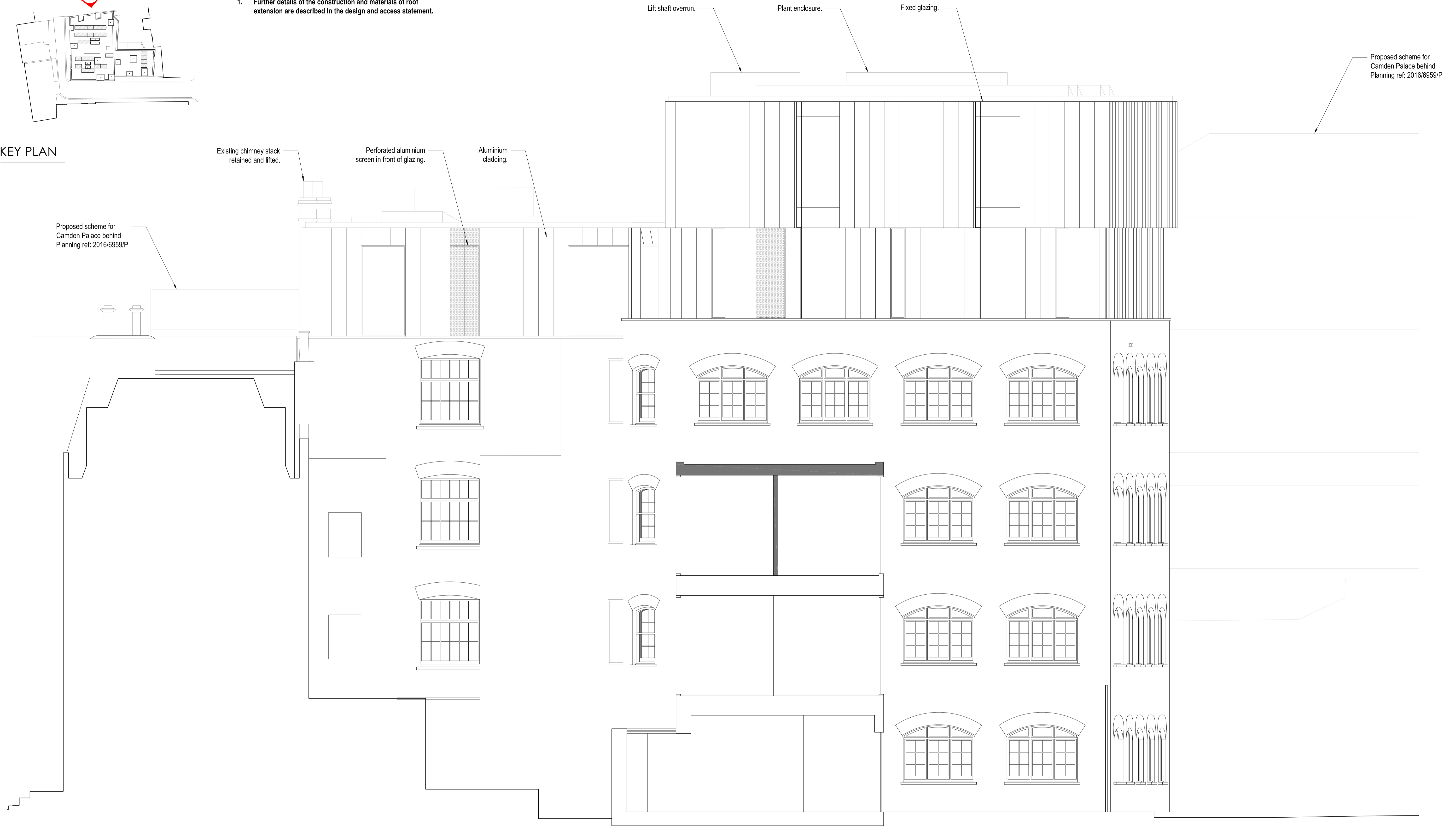
REAR ELEVATION
