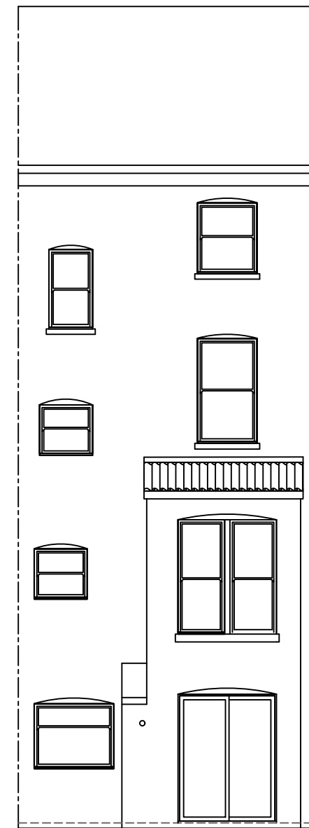
Rear Elevation
