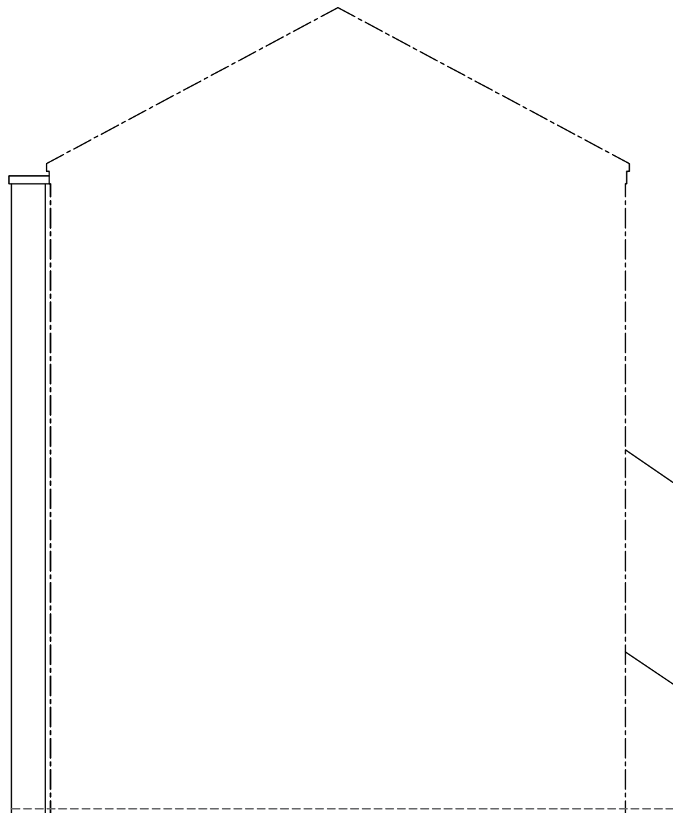
Left hand elevation - Viewed from rear of property
