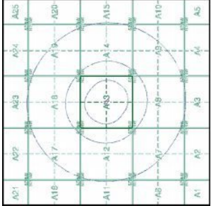
Borehole Map - Slice A
