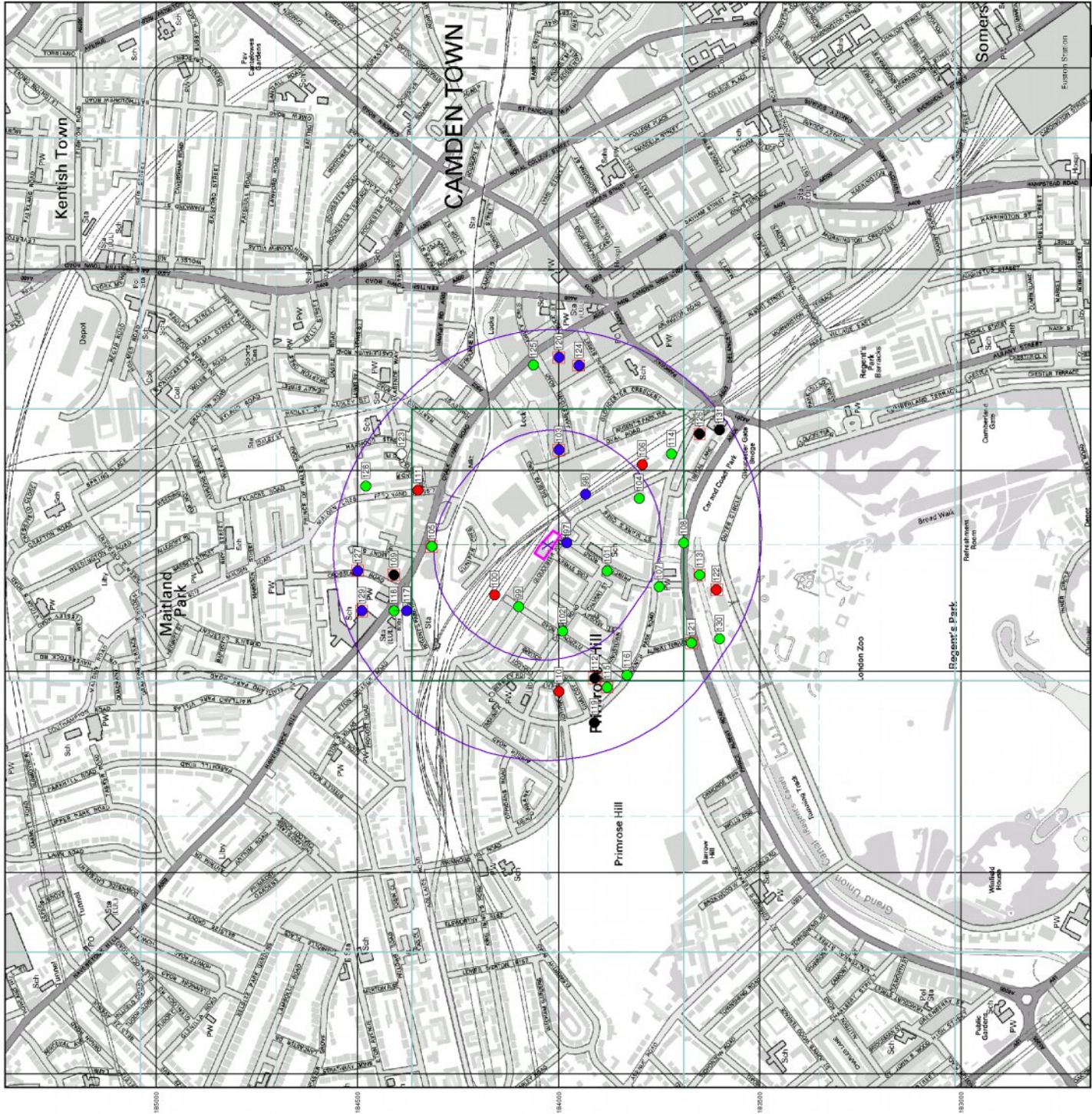
Borehole Map - Slice A
