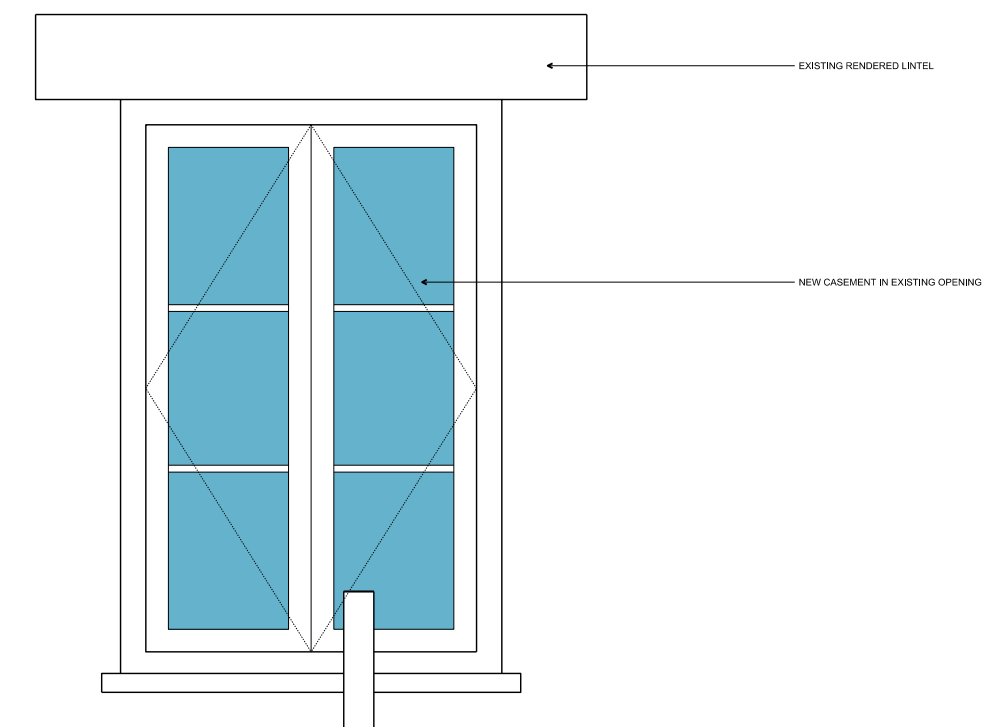
04 PROPOSED TYPICAL NARROW REAR CASEMENT WINDOW
