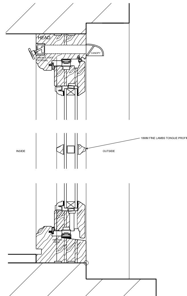
03 TYPICAL HEAD BAR AND CILL DETAILS
