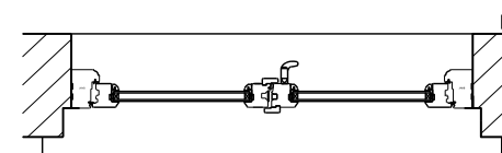
05 PROPOSED TYPICAL CASEMENT WINDOW TO CLOSET WING
