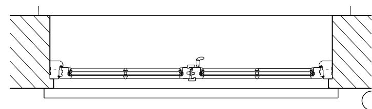
01 PROPOSED TYPICAL LARGE CASEMENT WINDOW
