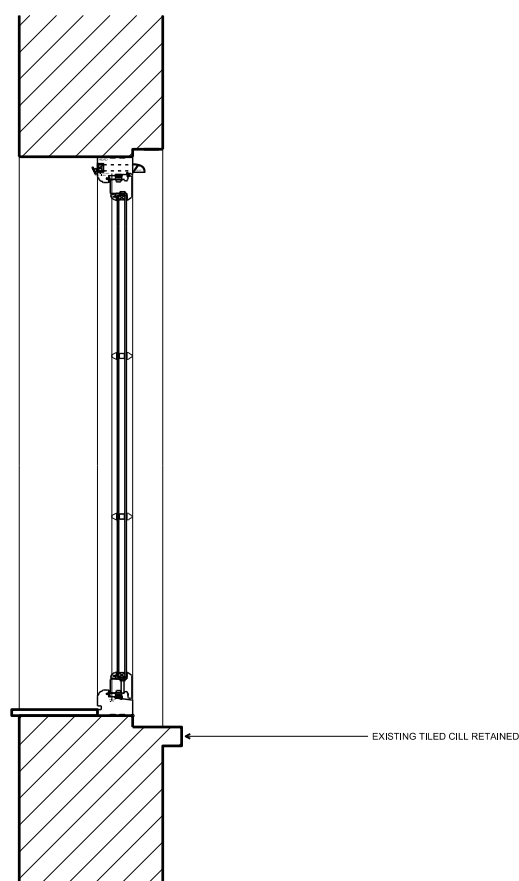
02 PROPOSED TYPICAL CASEMENT SECTION
