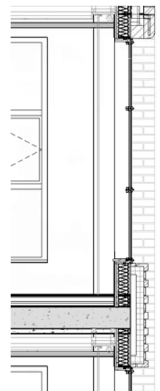
Typical Section of Window
