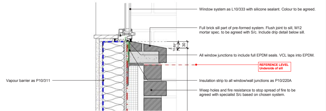
Cill Detail Scale 1:10
