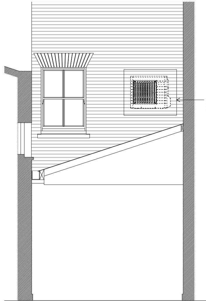
② NORTH ELEVATION 1:50 @ A3
