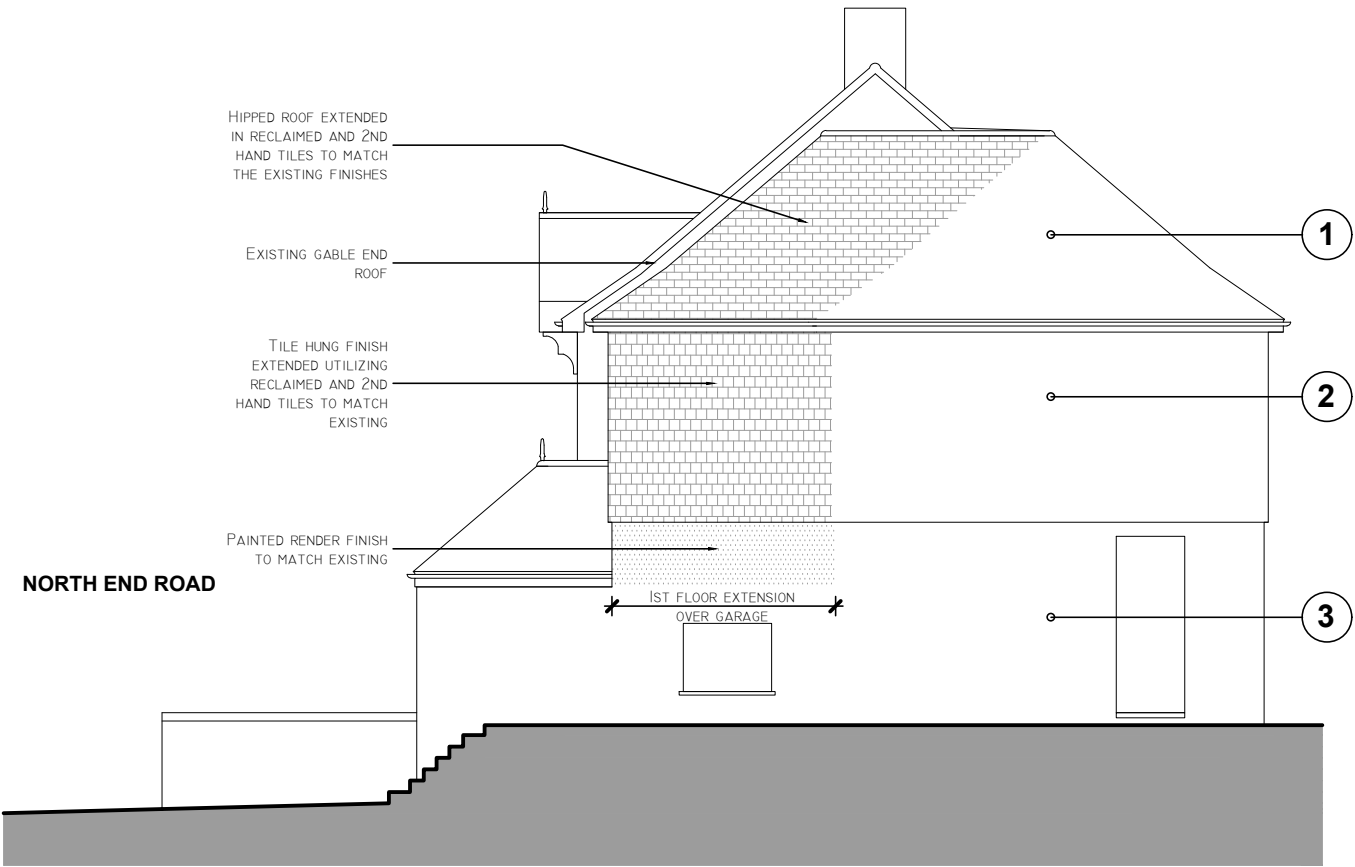
SIDE ELEVATION
