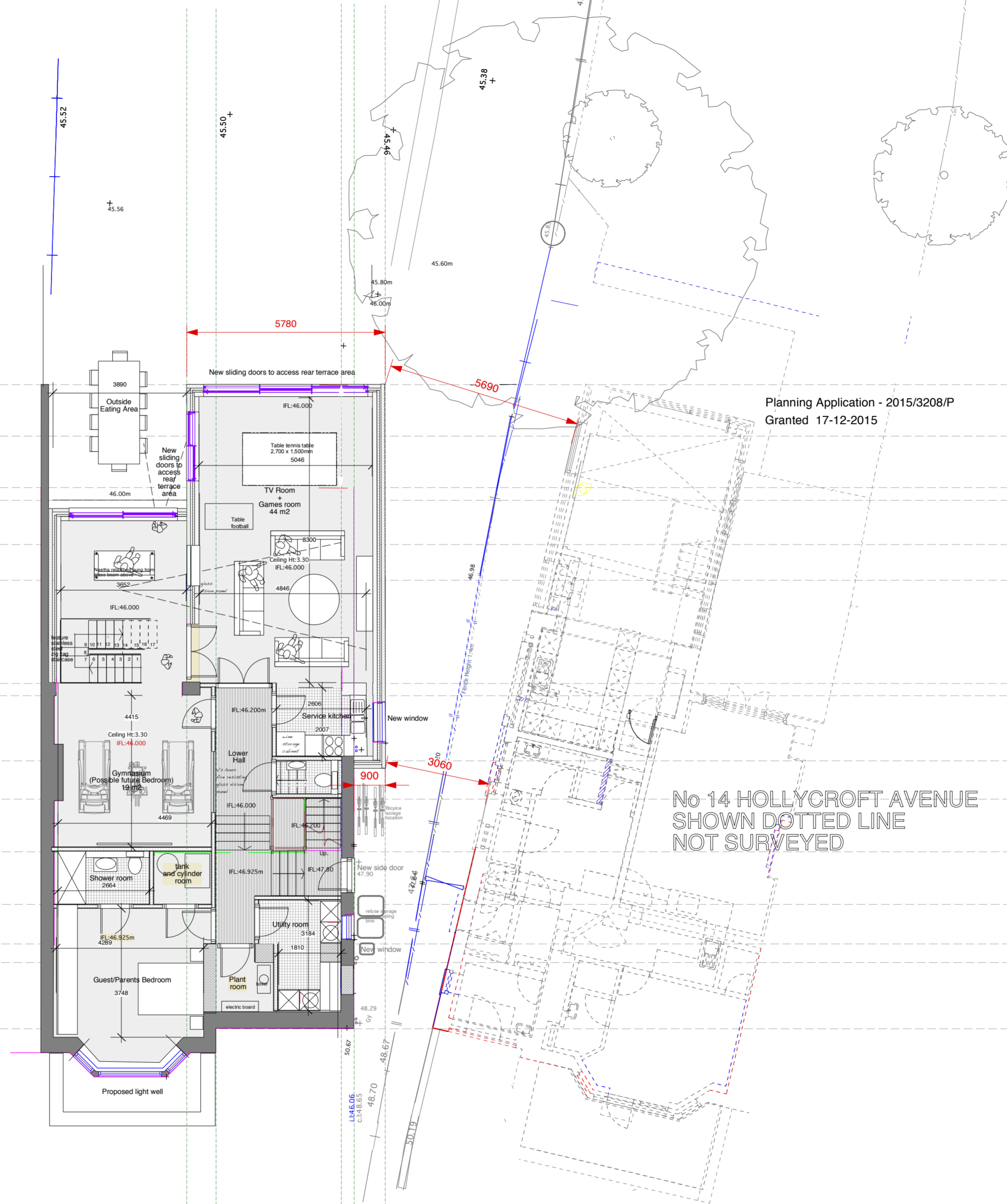
PROPOSED LOWER GROUND FLOOR
