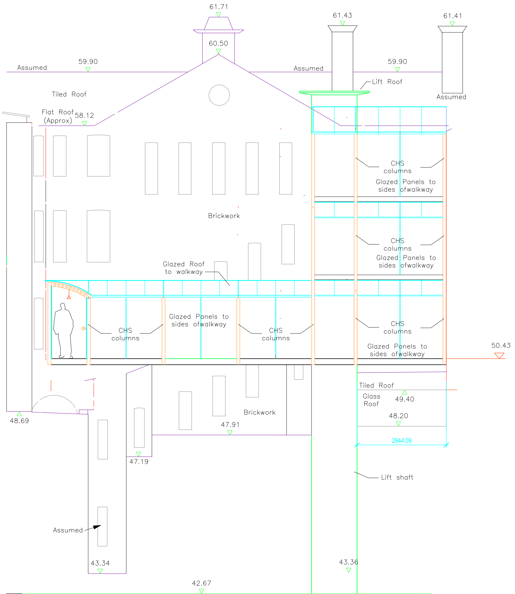
Northern Elevation Lightwell-Proposed
