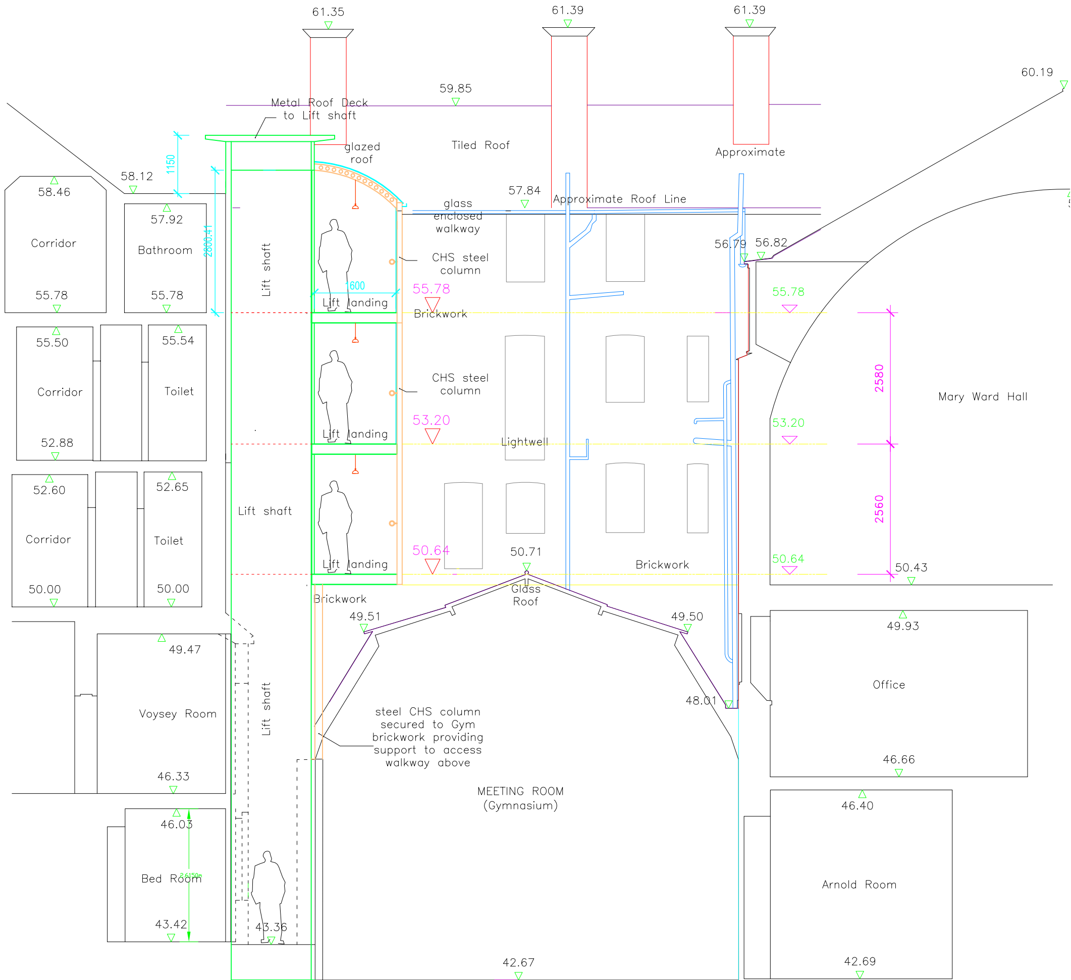
Section C-C / East Facing Elevation - Proposed
