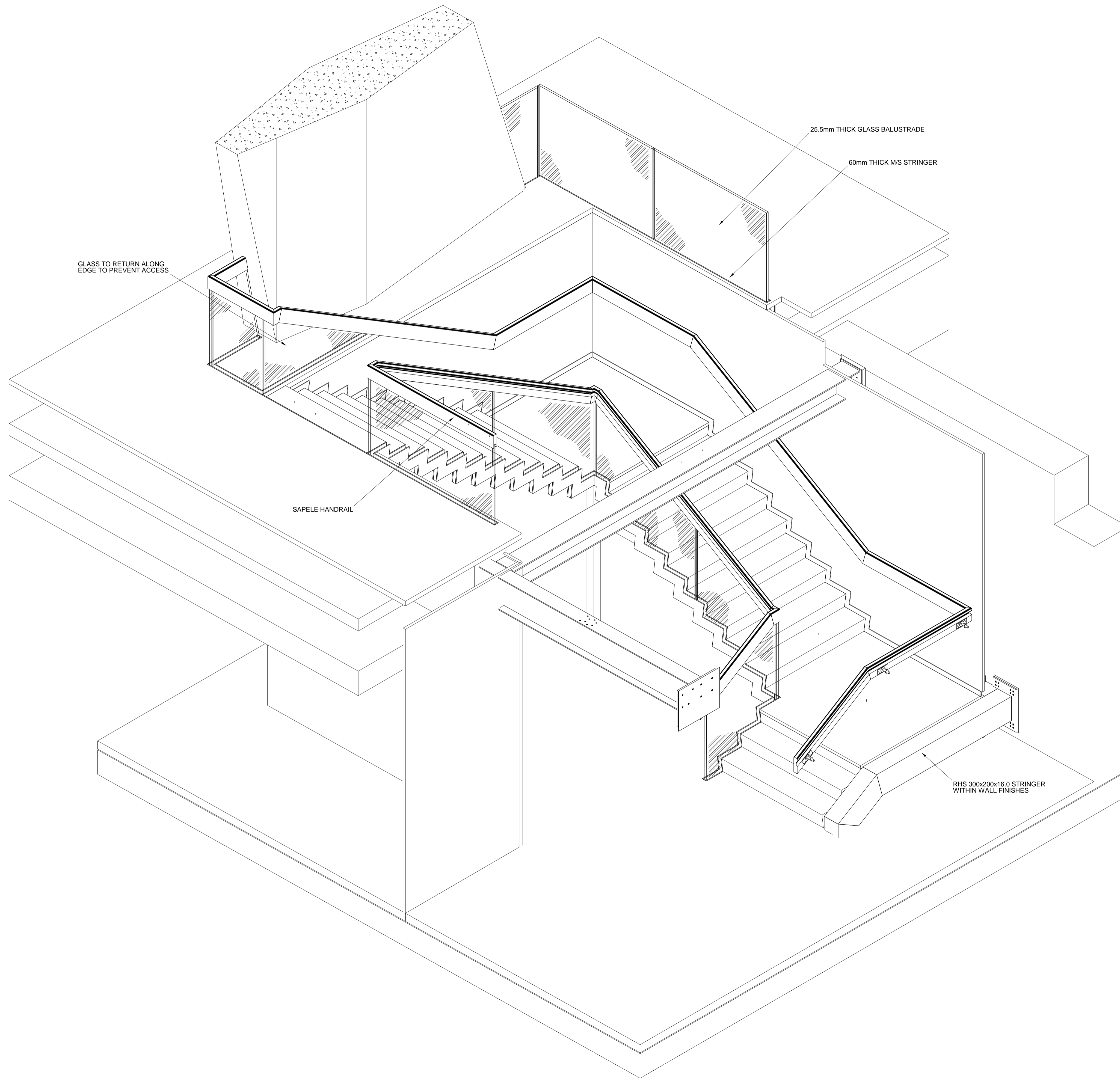
ISOMETRIC VIEW
