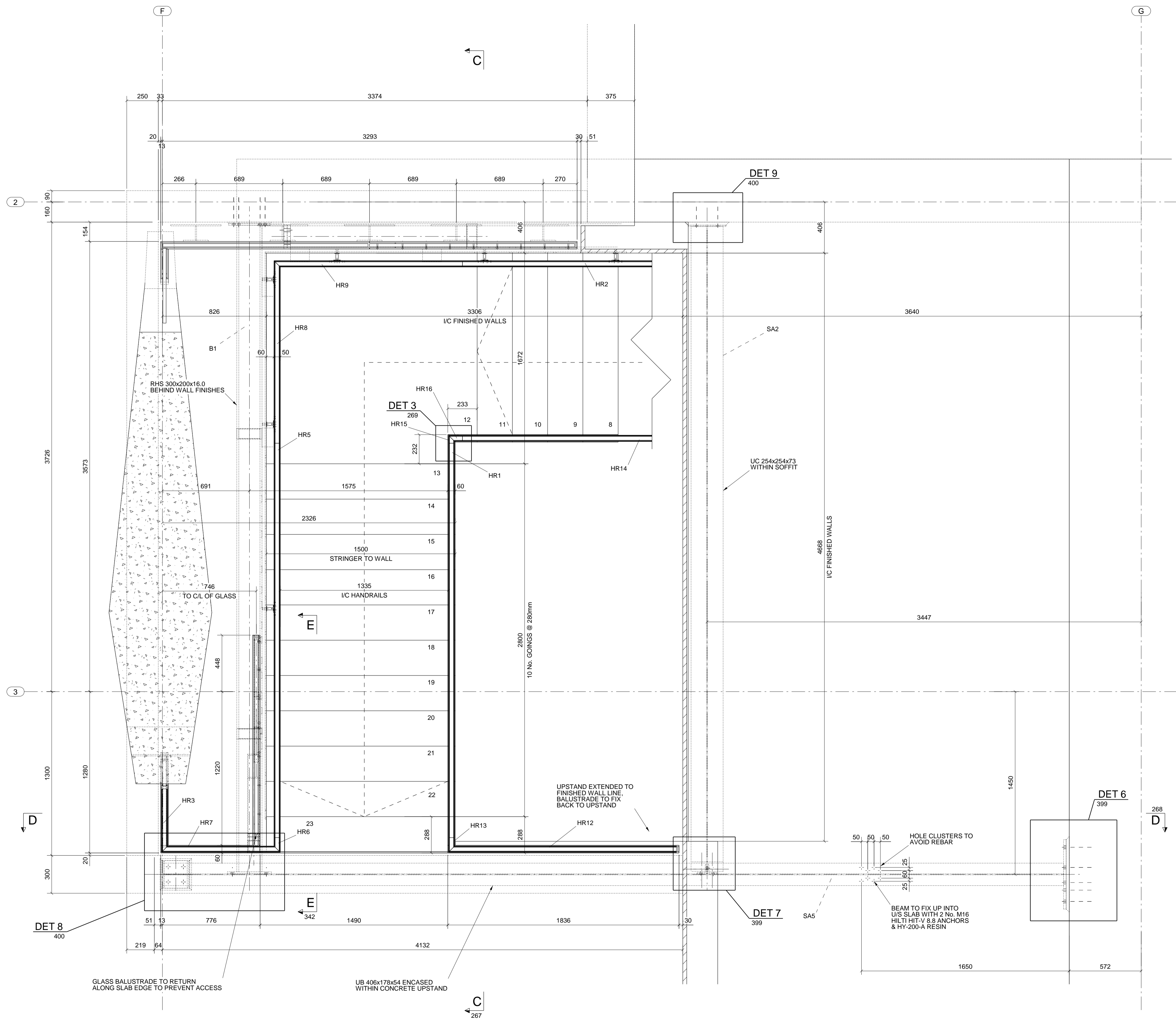
PLAN VIEW GROUND FLOOR FFL+25.600m
