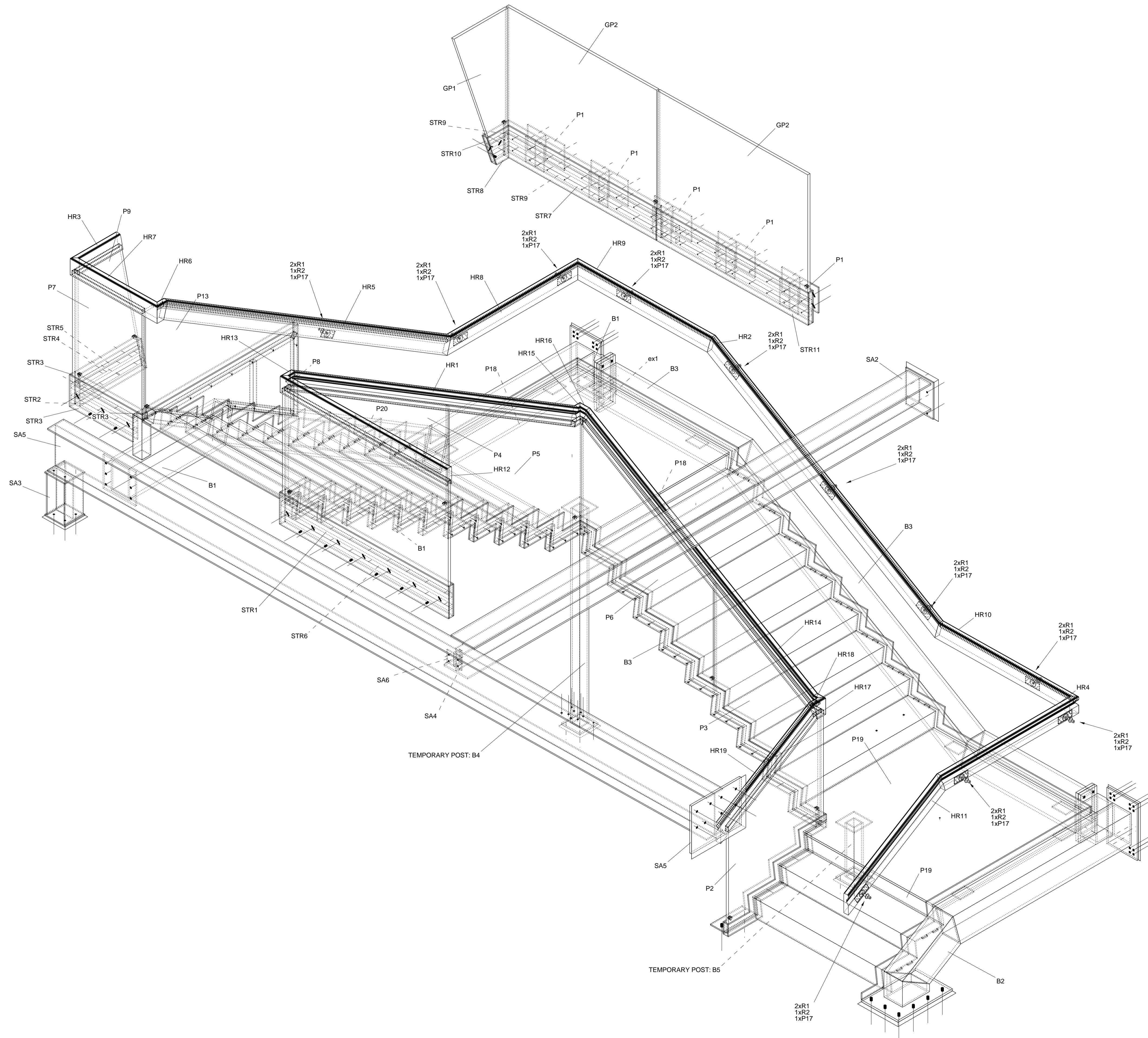
ISOMETRIC VIEW SECONDARY STEELWORK
