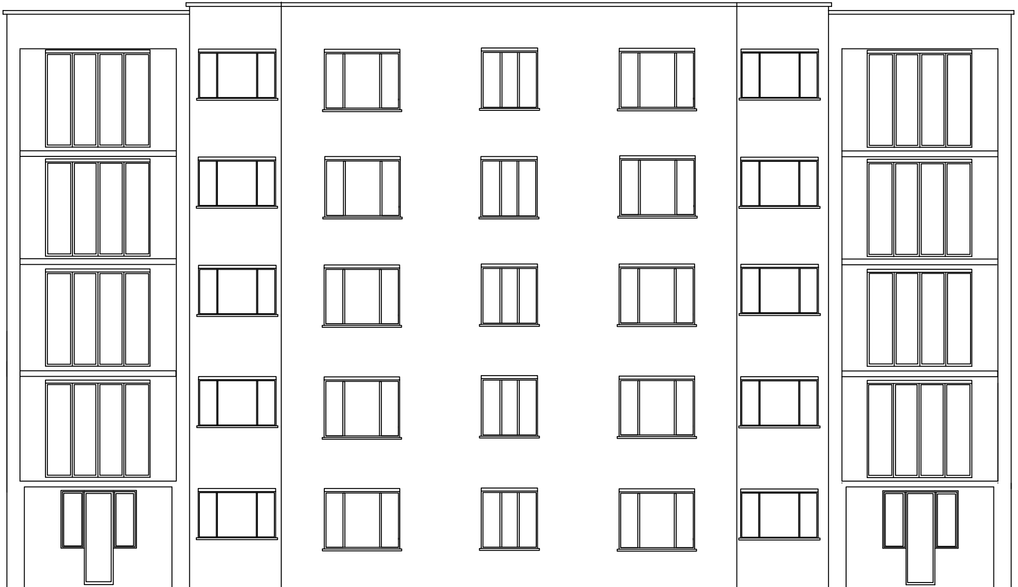
REAR ELEVATION - PROPOSED WINDOWS AND DOORS ARE TO BE DOUBLE GLAZED ALUMINIUM UNITS (COLOUR TO BE WHITE SHADE RAL NUMBER 9910 MATT)
