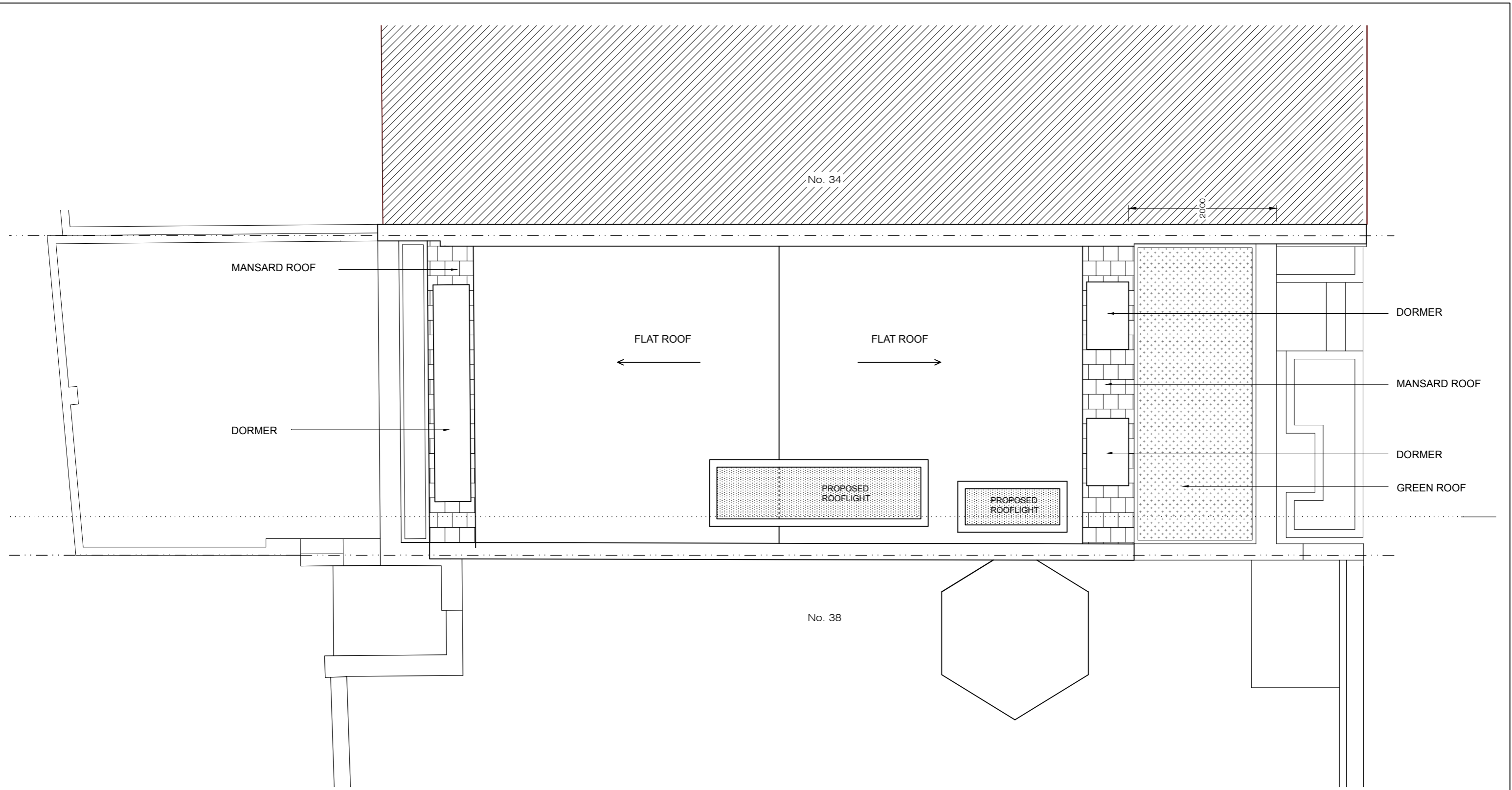
Proposed Revised Roof Plan 1:50 @ A3
