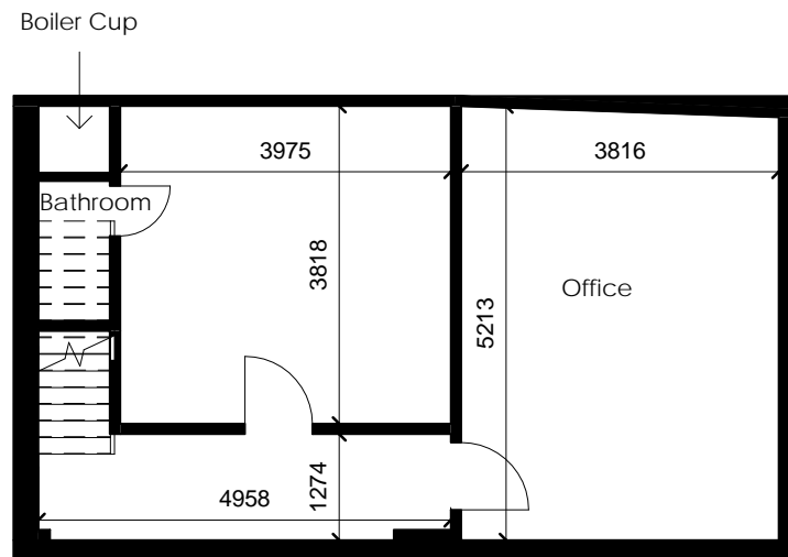
Existing Lower Ground Floor 1:100 @ A3 1:200 @ A4
