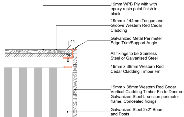
04 Vertical 'Roof Edge' Section 1:10
