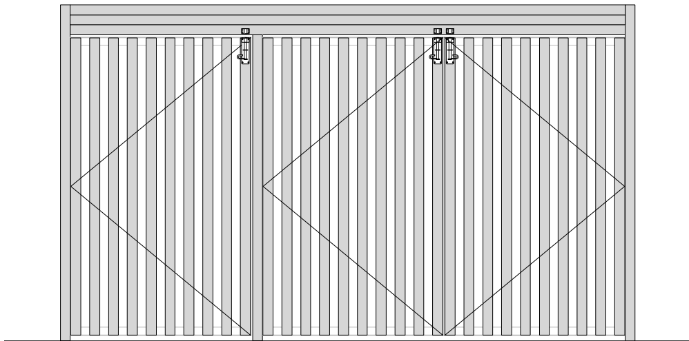
02 Front Elevation 1:20
