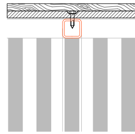
03 Vertical 'Roof' Section 1:10
