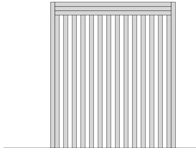
05 Side Elevation 1:20
