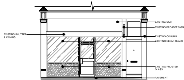
EXISTING SHOP FRONT SCALE 1:50
