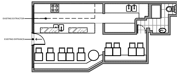
EXISTING GROUND FLOOR PLAN SCALE 1:50
