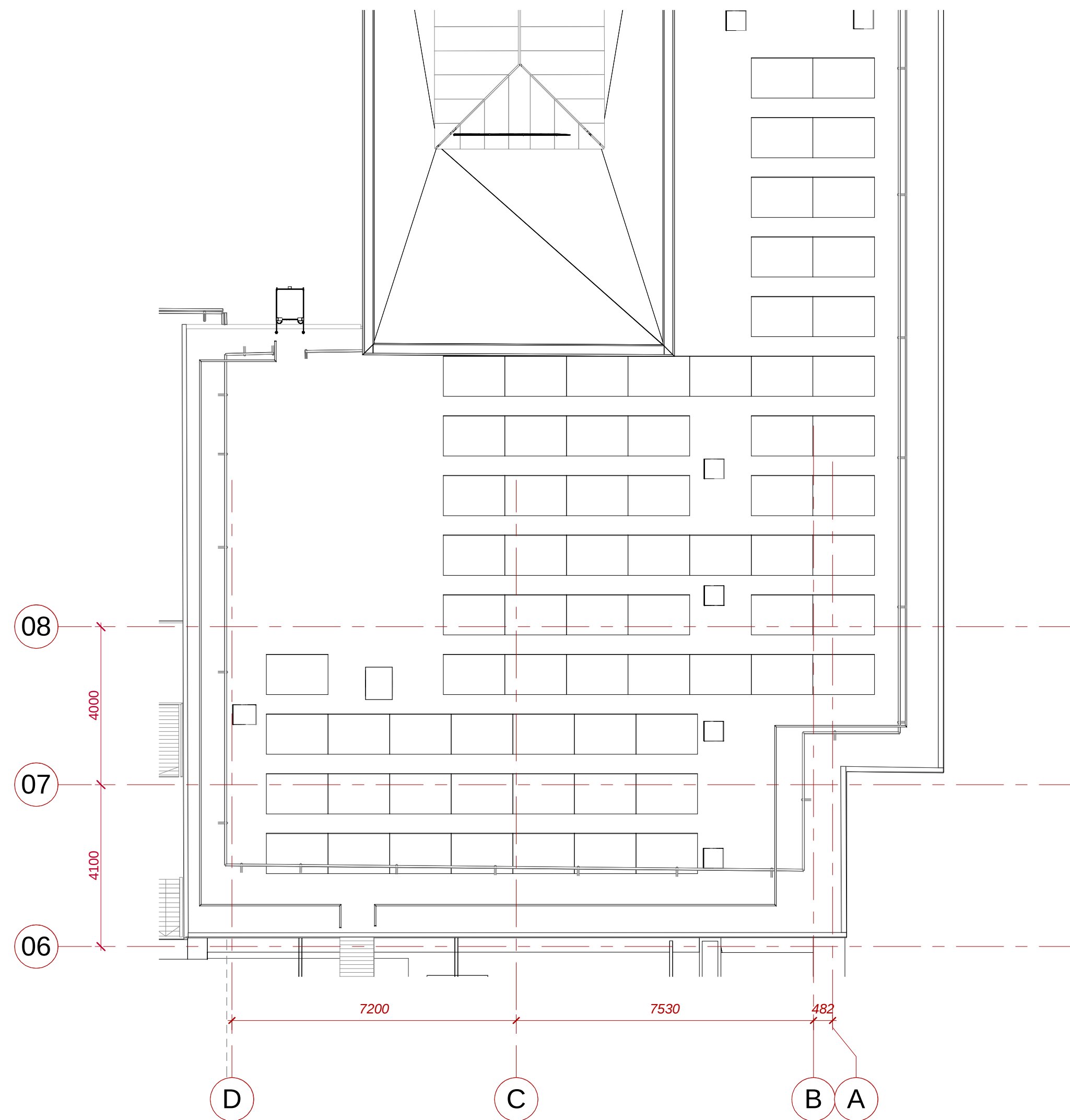
Photovoltaic Panel Layout on Bloomsbury Theater Roof
