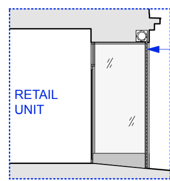
Section through entrance alcove
