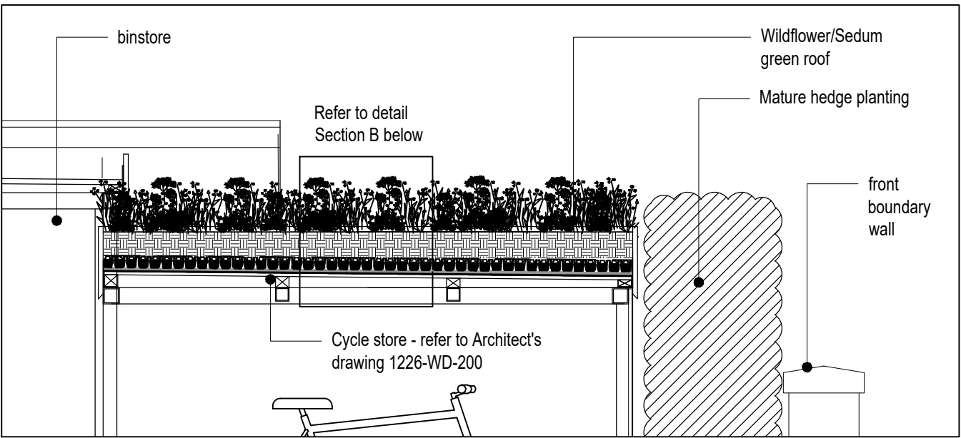
Section A: Cycle store green roof detail 1:20
