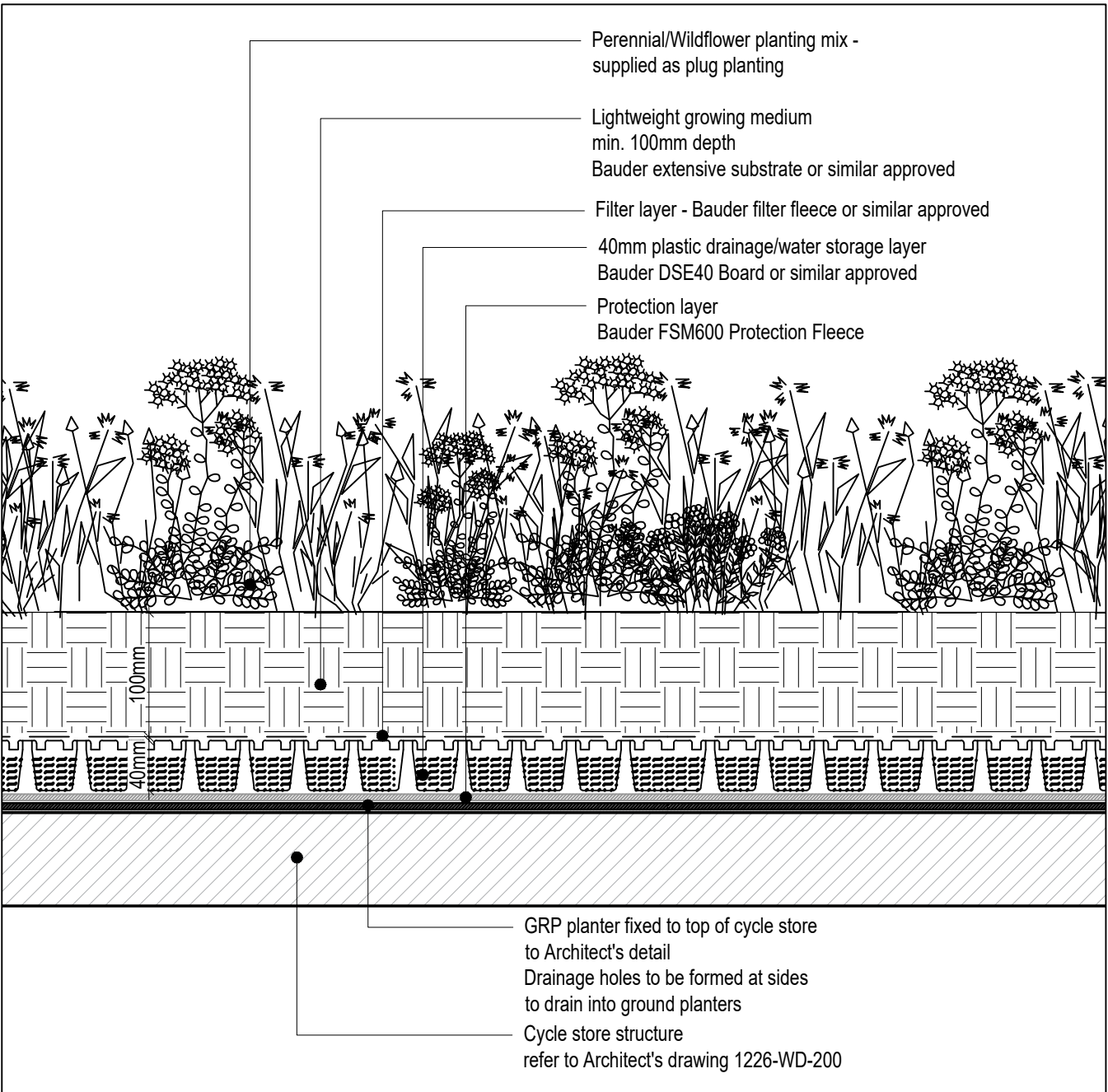
Section B: Cycle store green roof detail 1:5
