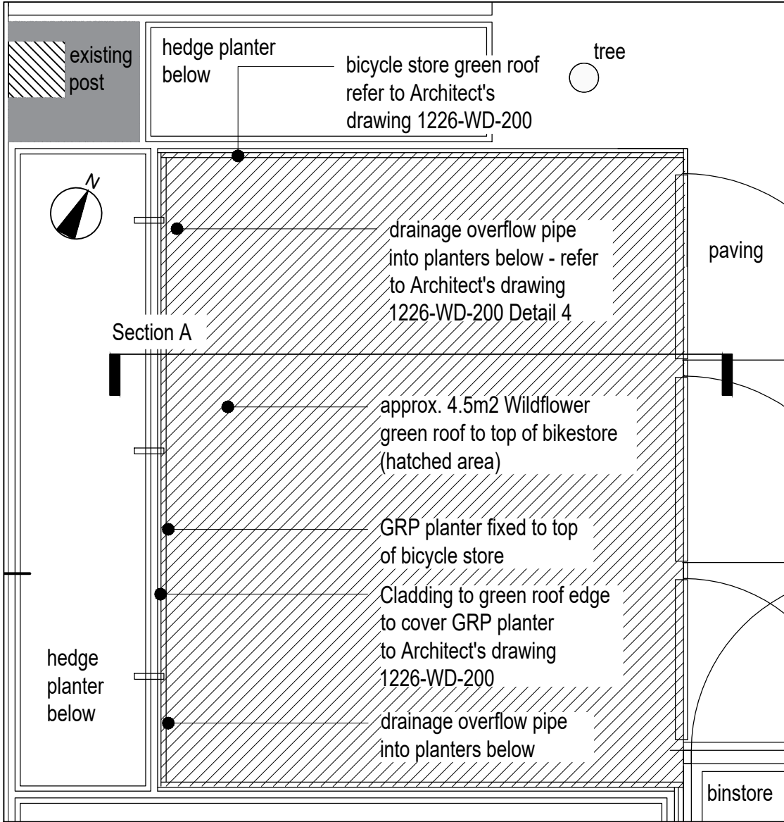
Plan A: Cycle store Green Roof 1:20
