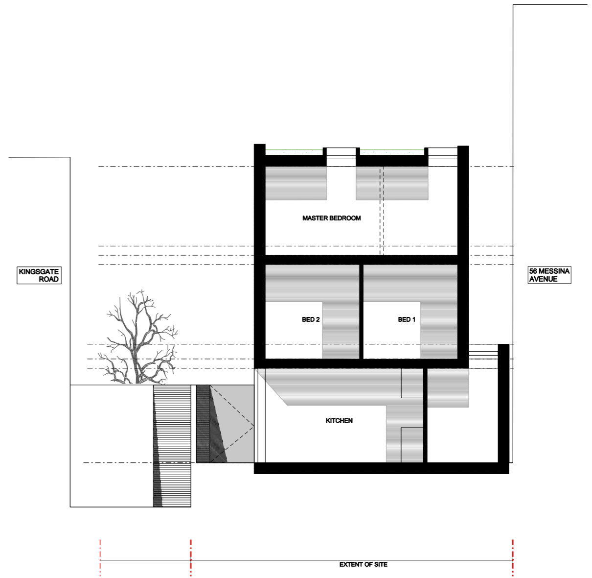
PROPOSED SECTION
