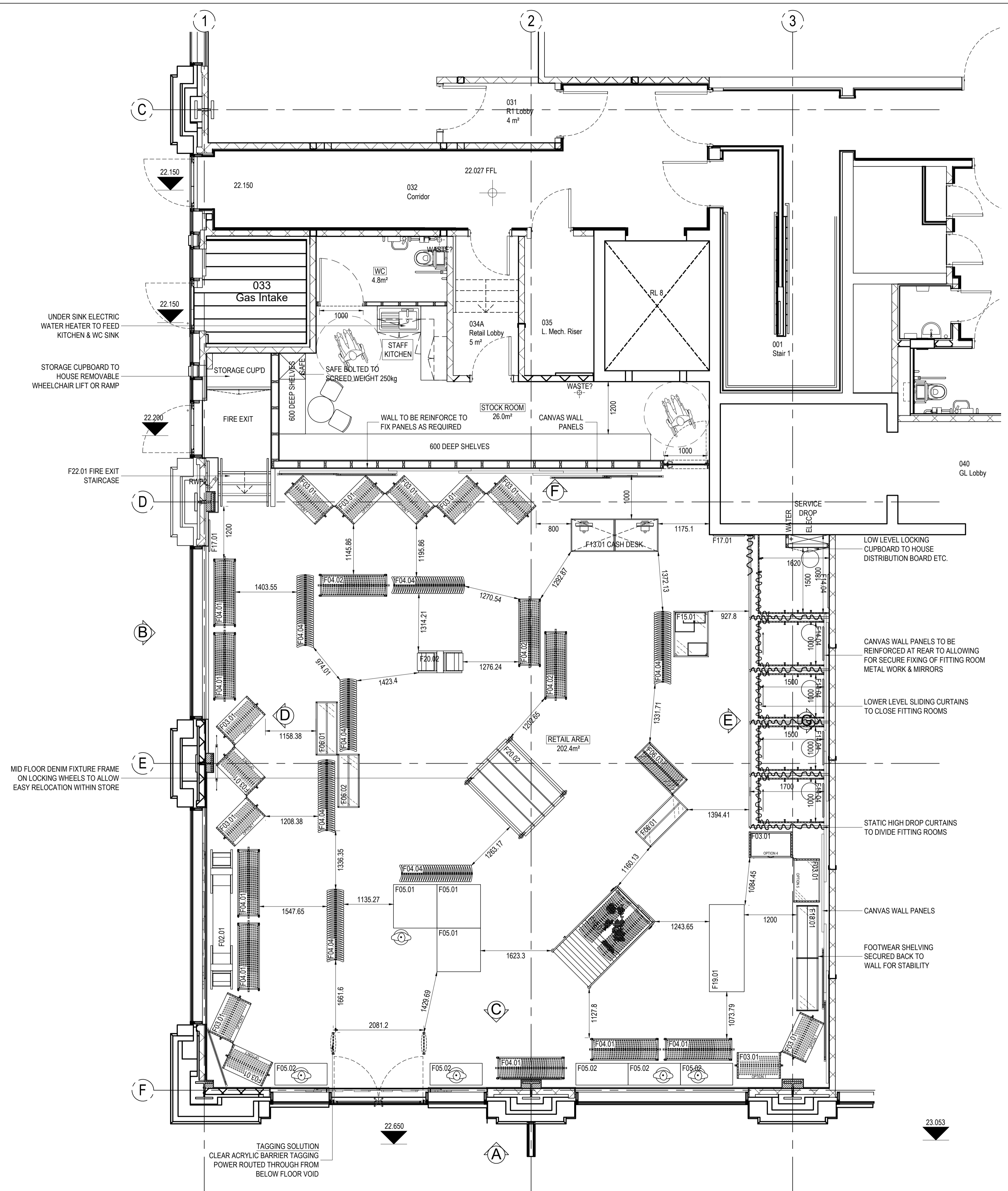
PROPOSED PLAN LAYOUT - GROUND FLOOR RETAIL SCALE 1:50
