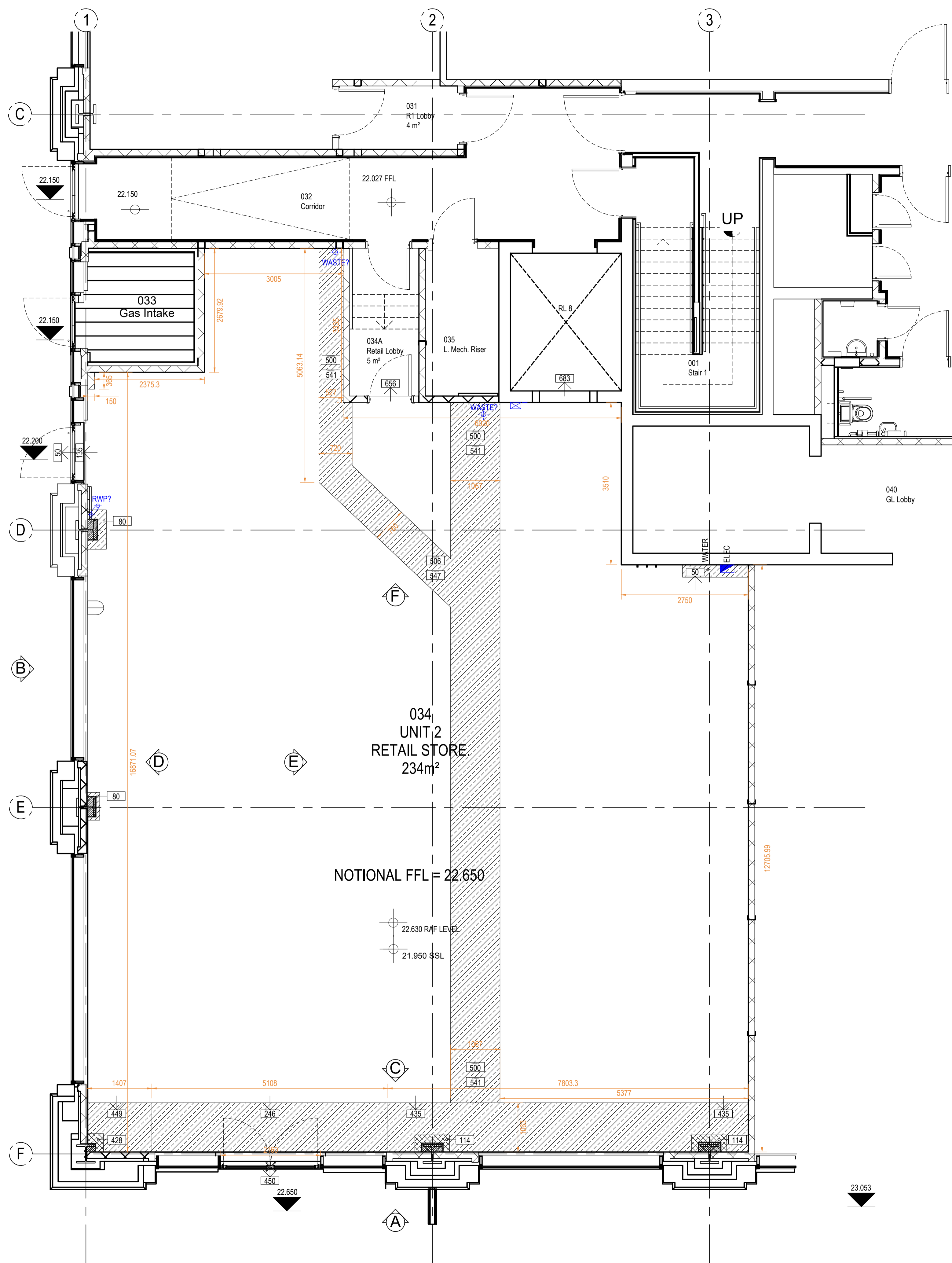
EXISTING PLAN LAYOUT SCALE 1:50
