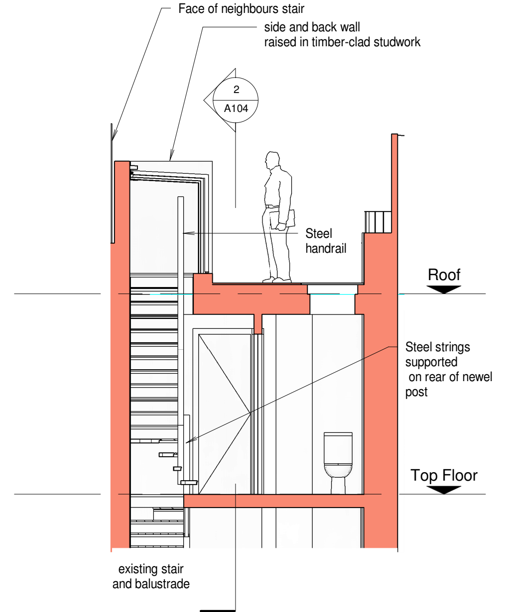
1 Section A - as Proposed 1 : 50
