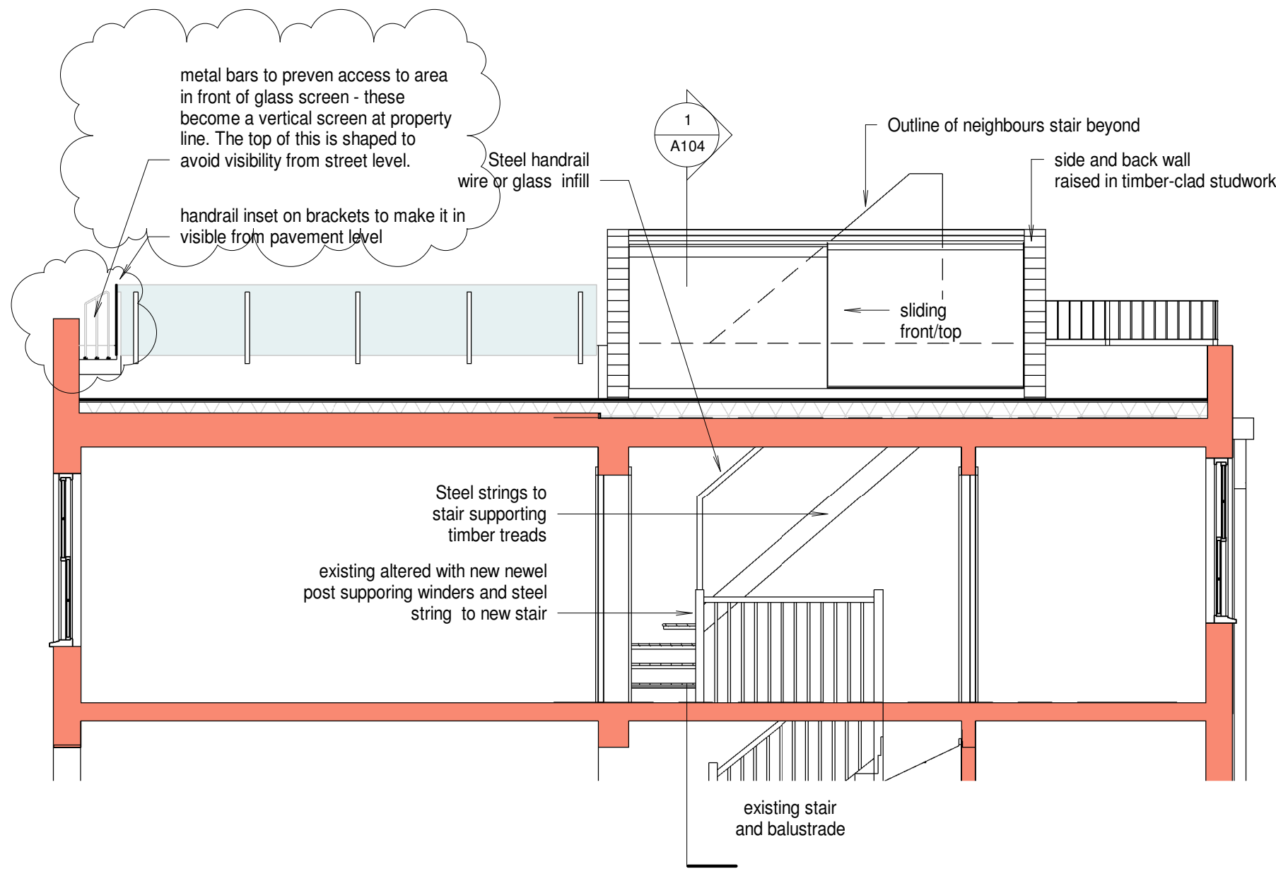
2 Section B - as Proposed 1 : 50
