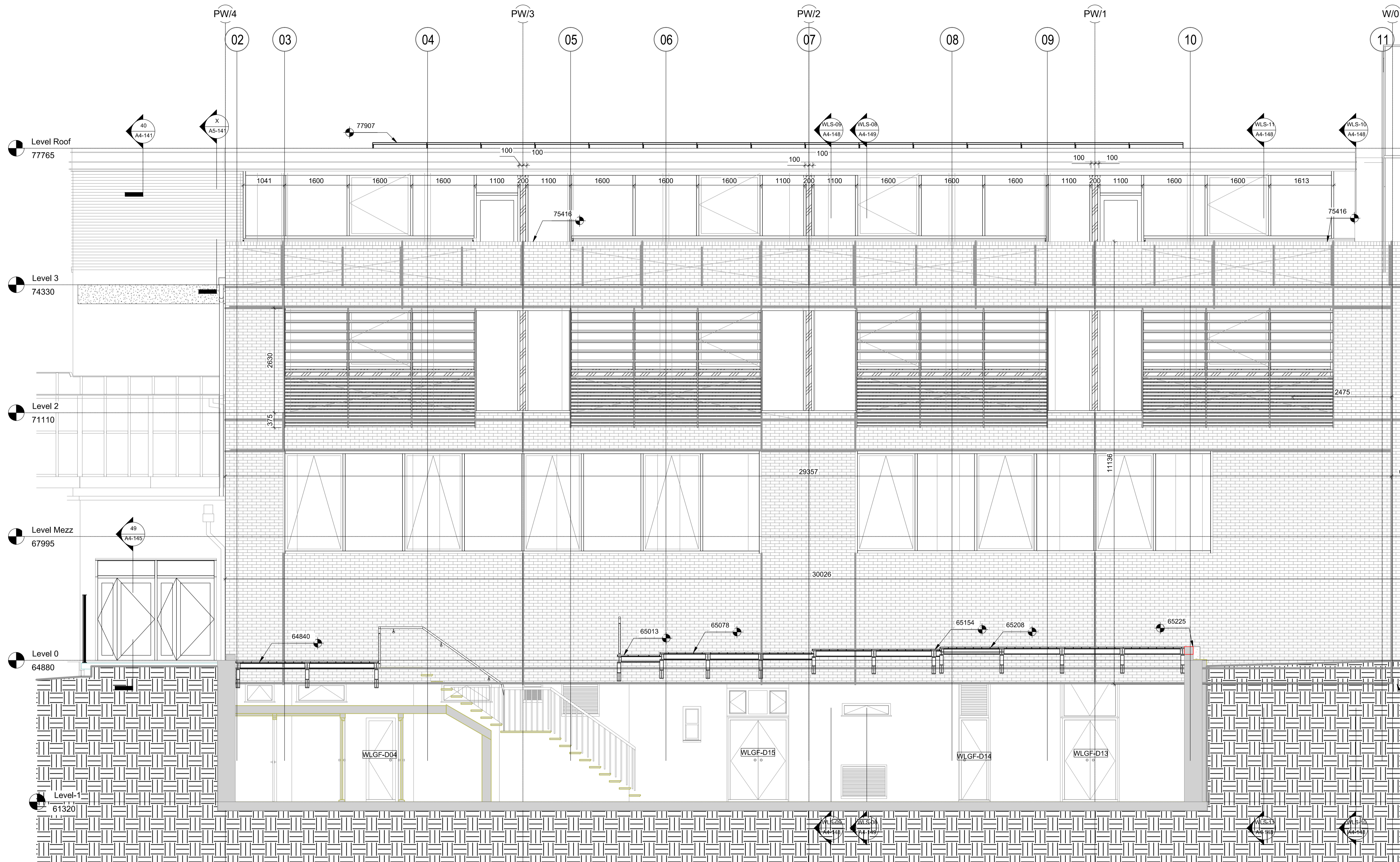
Elevation A (North) Scale 1:50@A1, 1:100@A3
