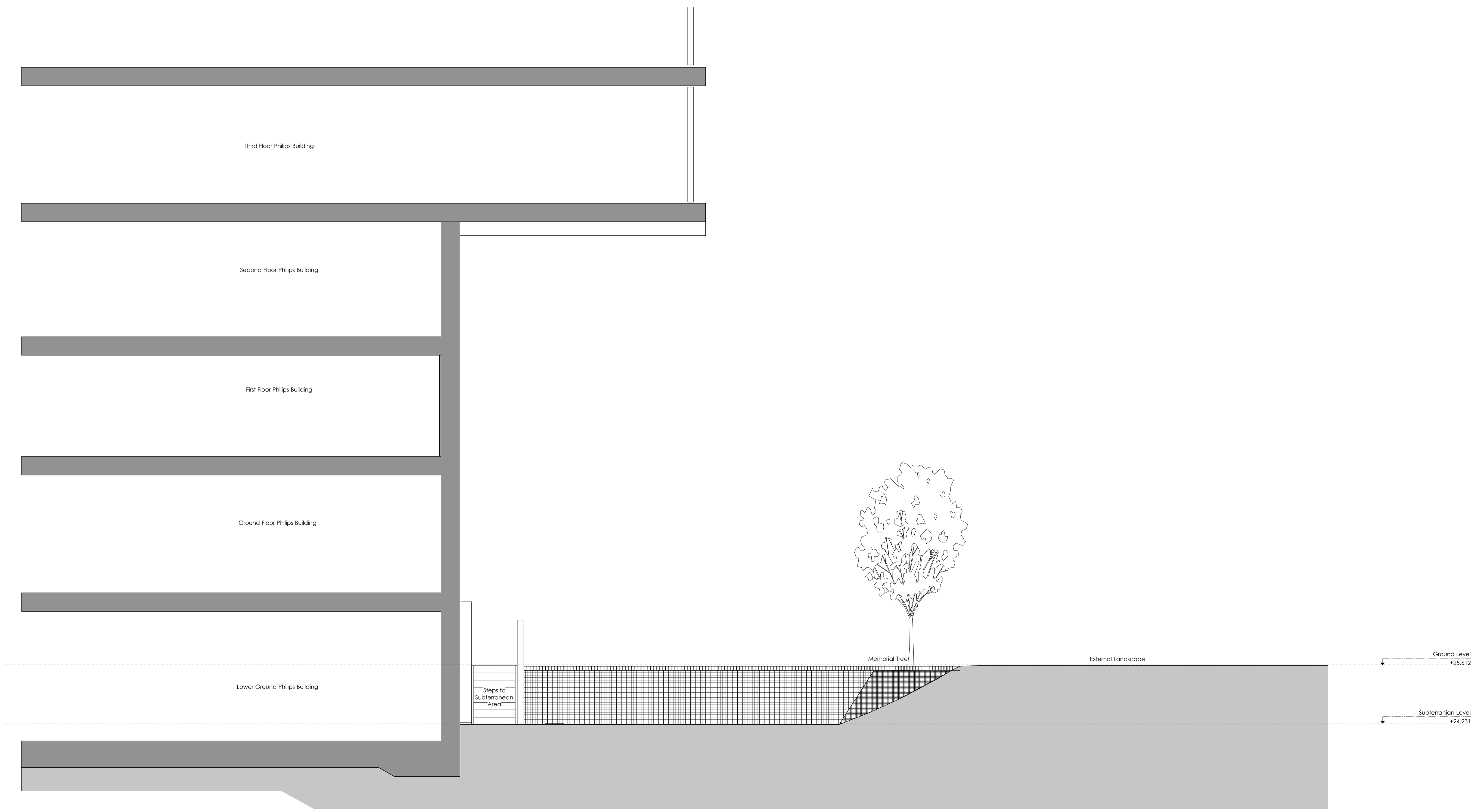
1 SOAS Philips Building-Existing Section C-C Scale: 1:50
