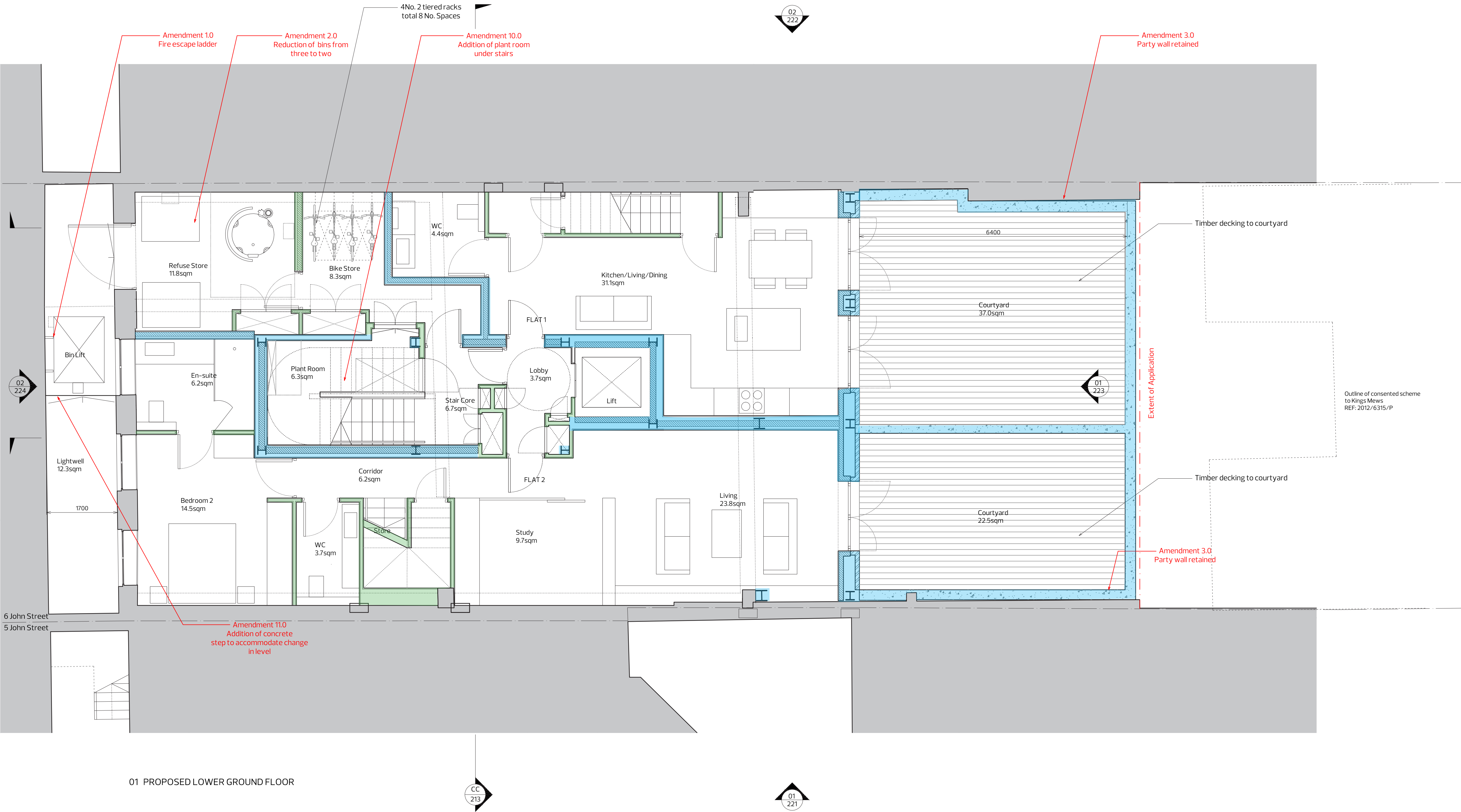
Lower Ground Floor Plan 1:100 @ A1 Consented 2015/3149/P by Coffey Architects
