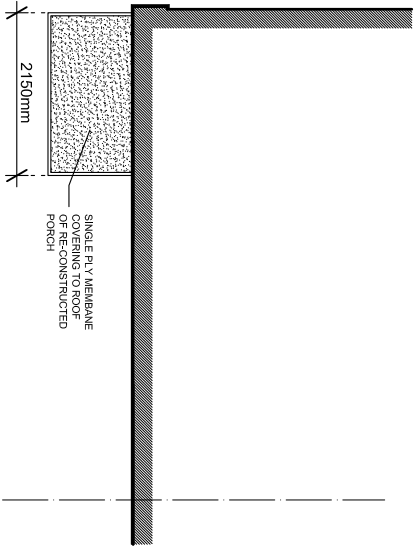
PLAN OF PORCH ROOF
