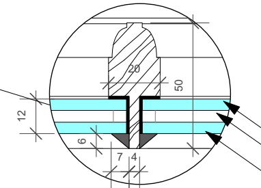
2B PLAN DETAIL - TIMBER GLAZING BAR SCALE 1:2@A3
