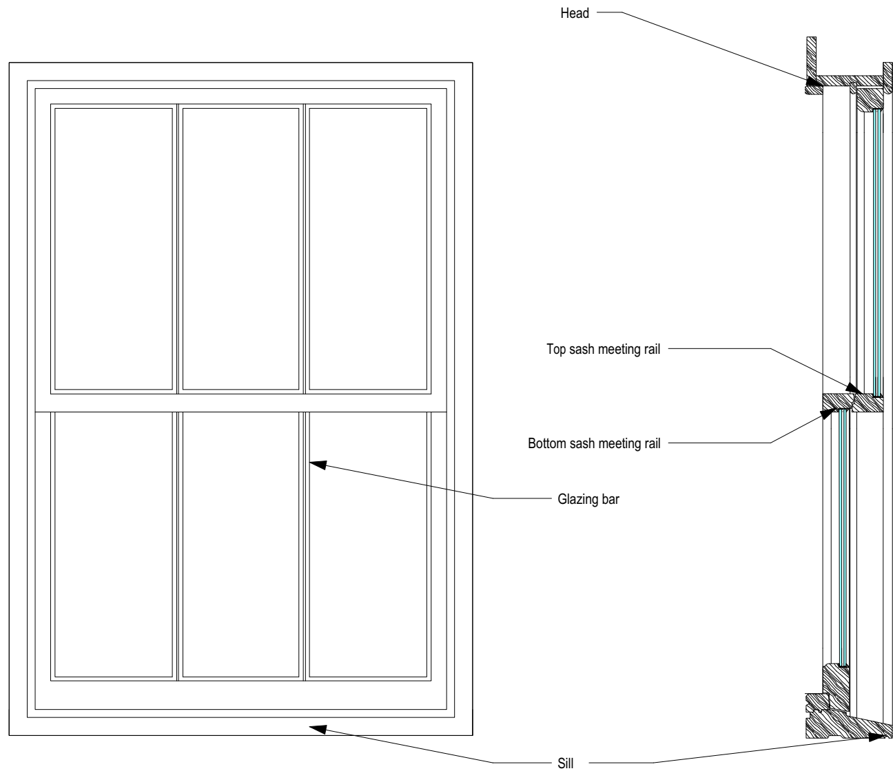
2C ELEVATION - GROUND FLOOR FRONT WINDOW SCALE 1:10@A3
