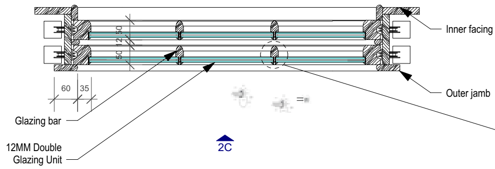
2A TYPICAL SASH WINDOW PLAN - GROUND FLOOR FRONT WINDOW SCALE 1:10@A3
