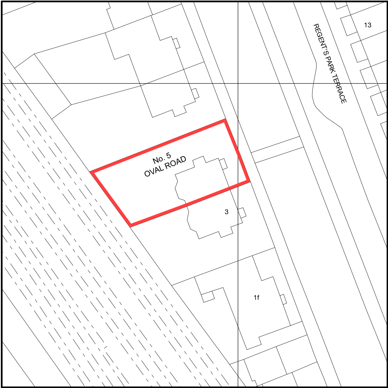
BLOCK PLAN
