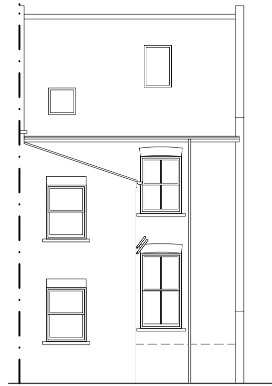
Existing Rear Elevation - South
