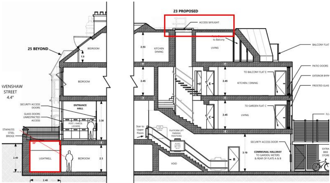
Figure 5: Light Wells and Skylight Location
