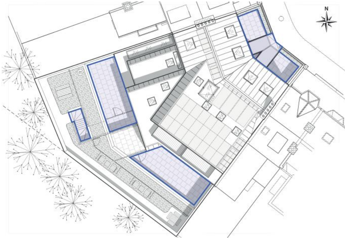
Figure 15: Areas with Impermeable Paving (90.14m 2 ) and not subject to water harvesting
