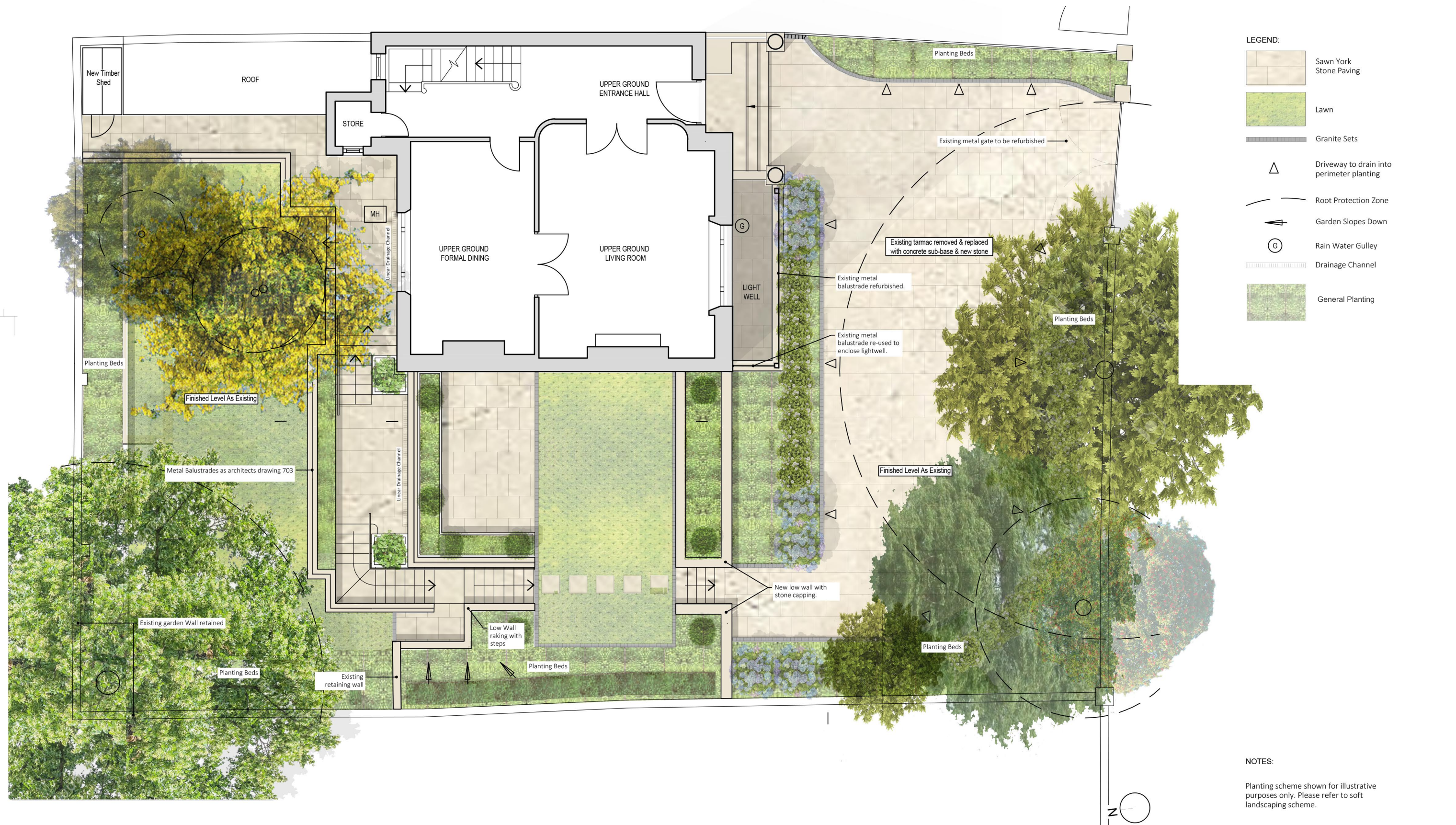
1 Landscape Design - ground floor plan 1:100
