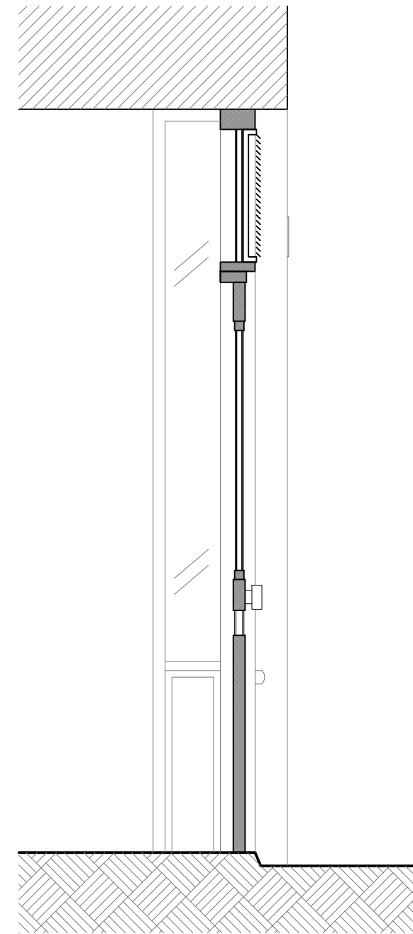
3 Existing Section 1:20
