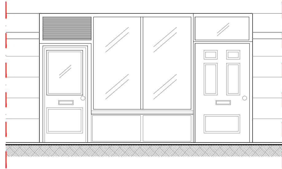
1 Existing Elevation 1:50
