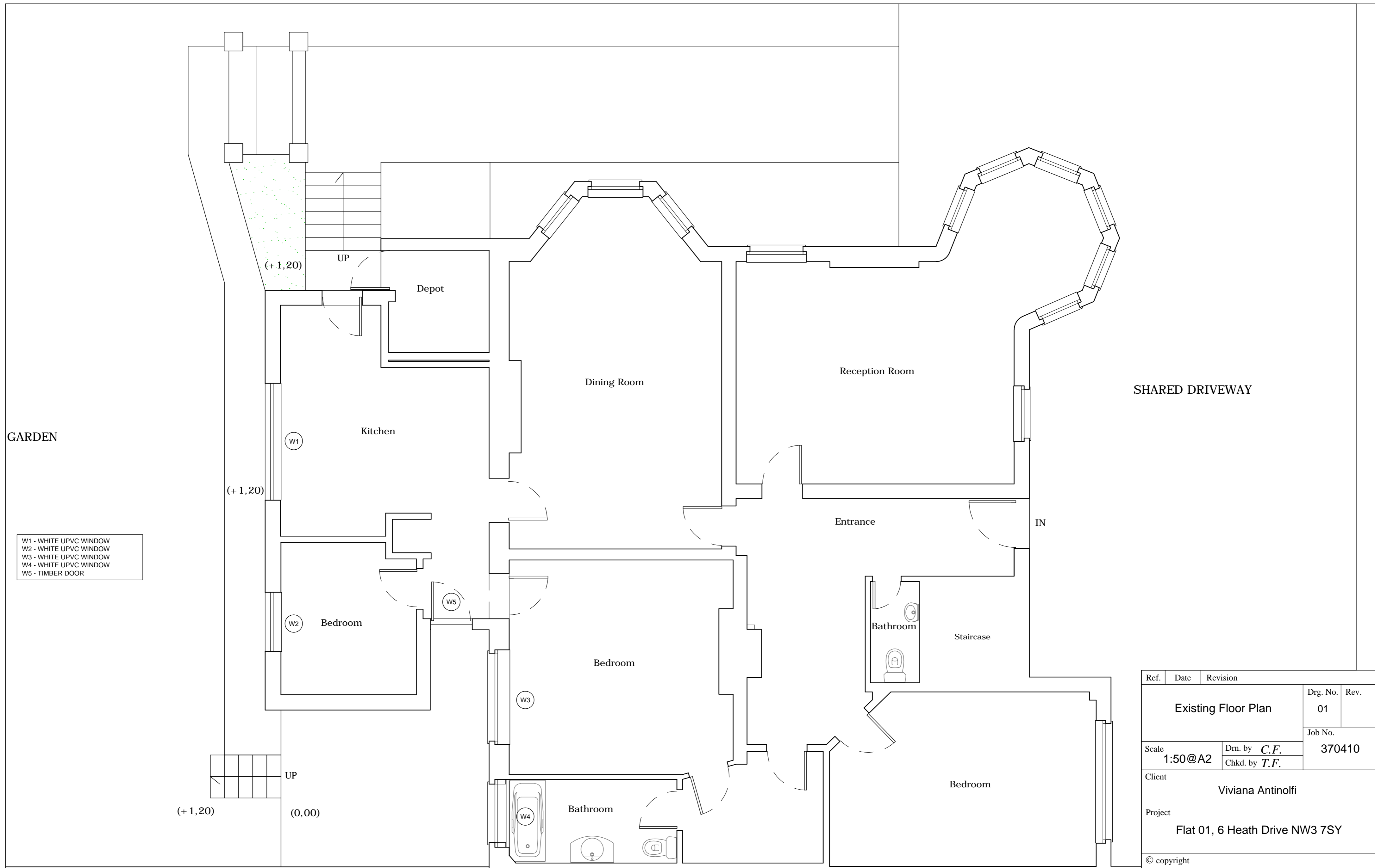
HEATH DRIVE - LONDON NW3 Existing Ground Floor Plan
