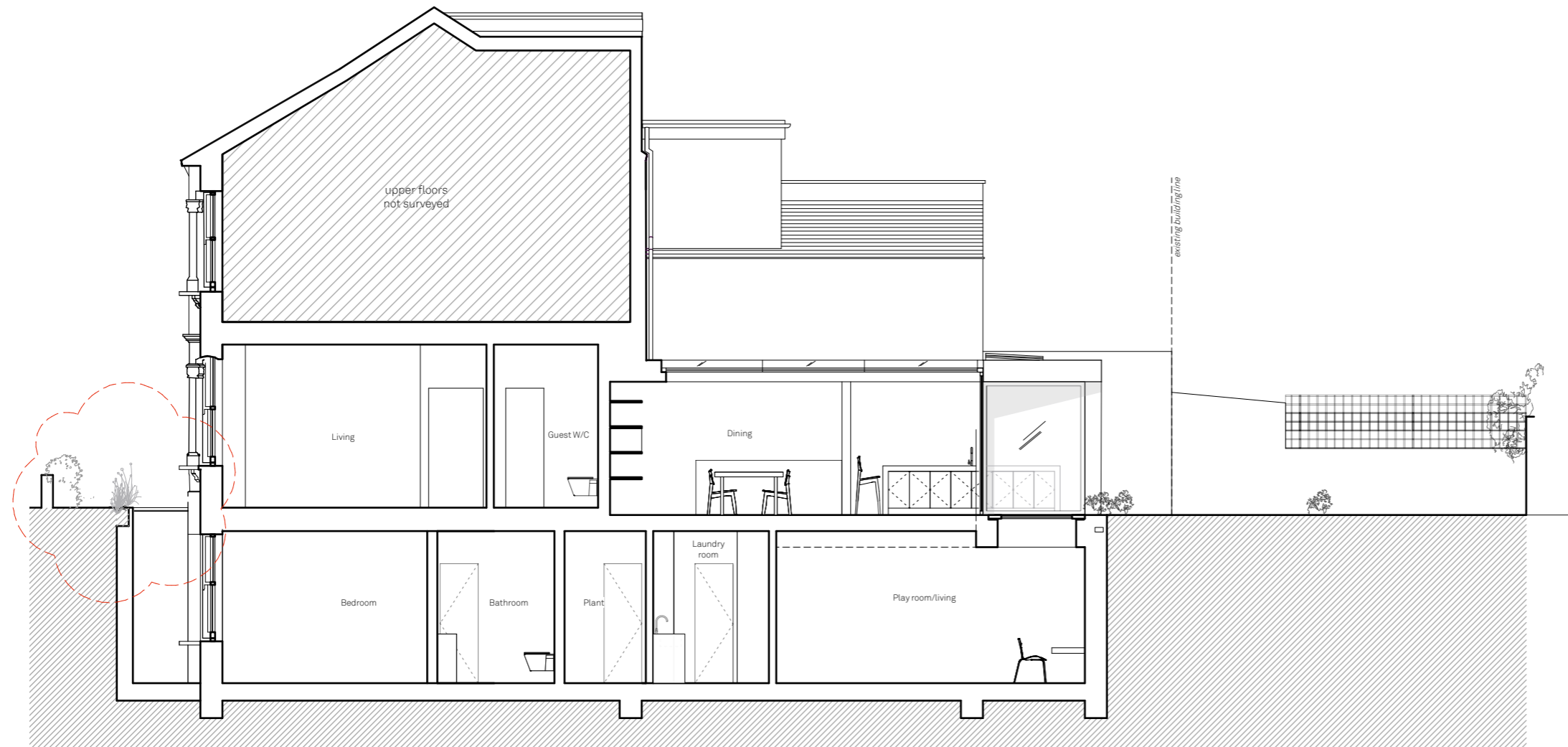
Section AA
