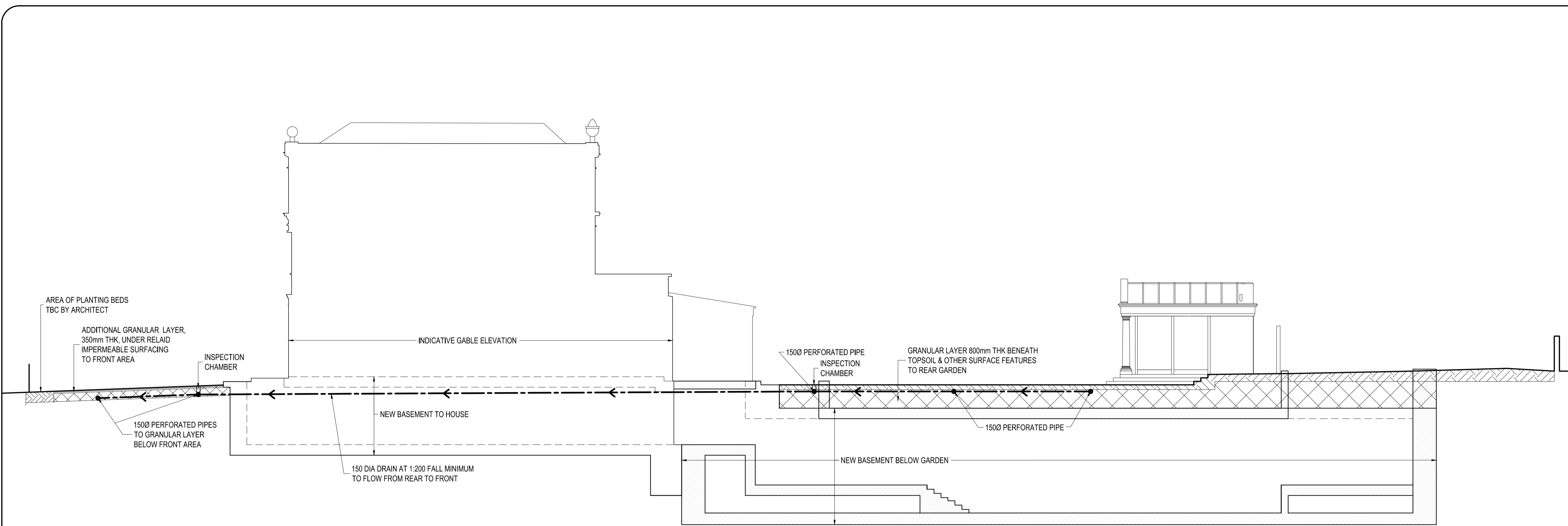
SECTION C-C: LONG SECTION SHOWING NEW PERMEABILITY PROPOSALS & DRAINS SCALE 1:100
