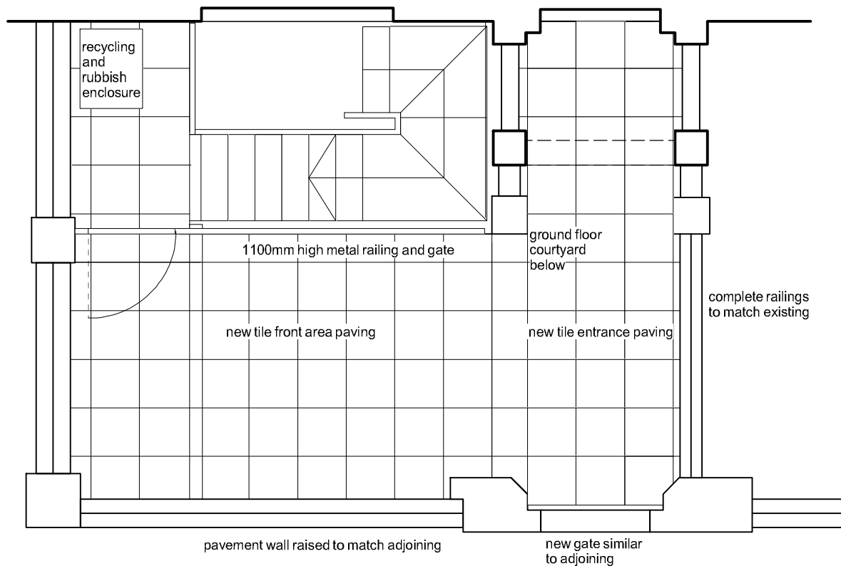
proposed plan
