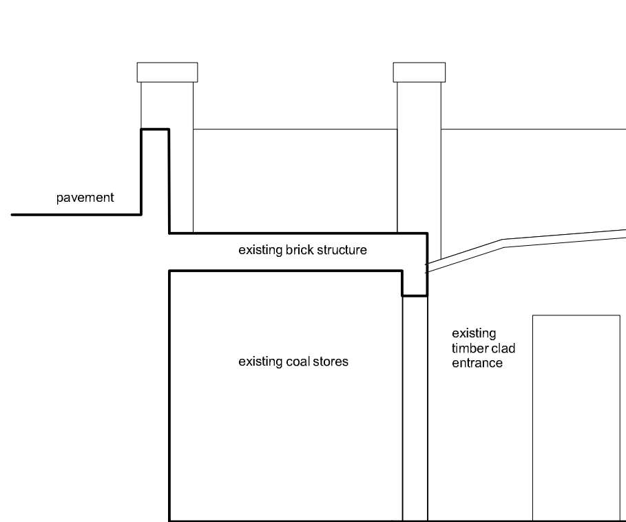
existing section
