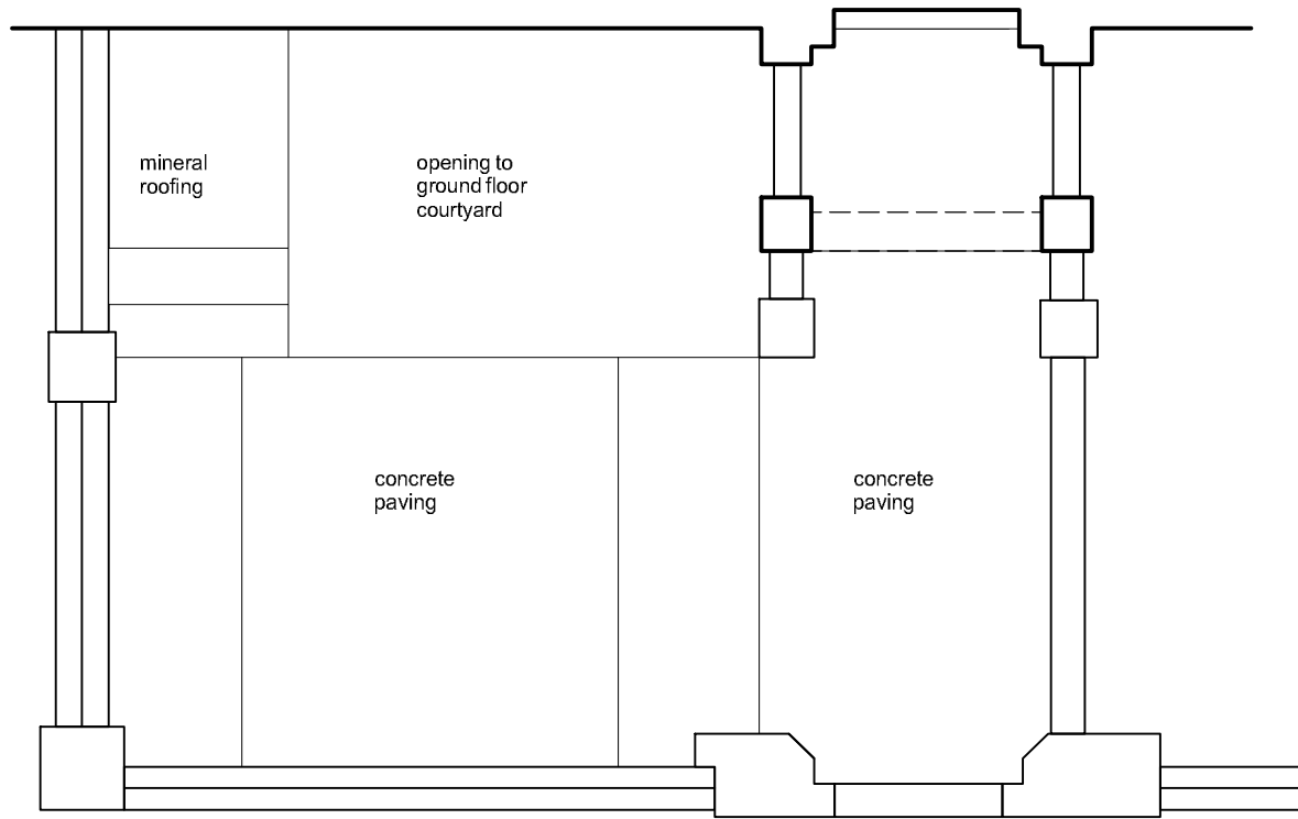
existing plan
